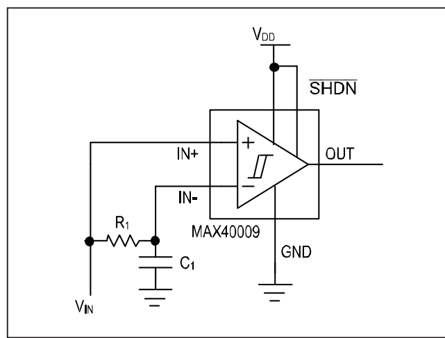
Figure 3. Time Averaging of the Input Signal for Data Recovery
