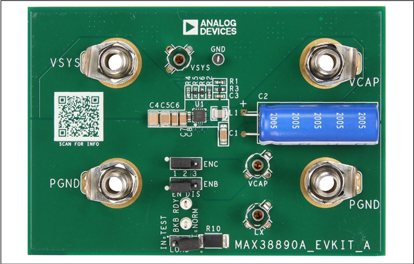
MAX38890A EV Kit Photo
