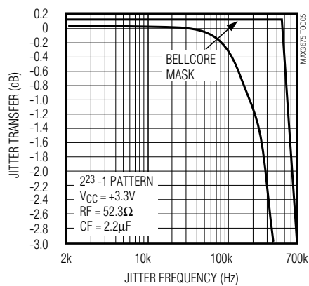
JITTER TRANSFER
