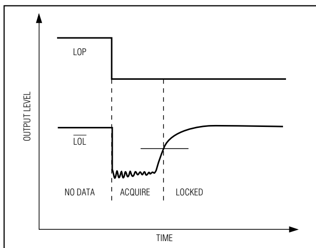
Figure 4. Loss-of-Lock Output
