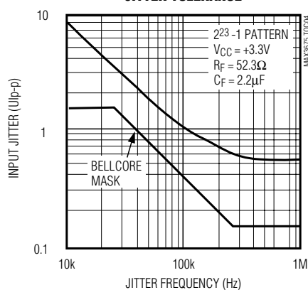
JITTER TOLERANCE
