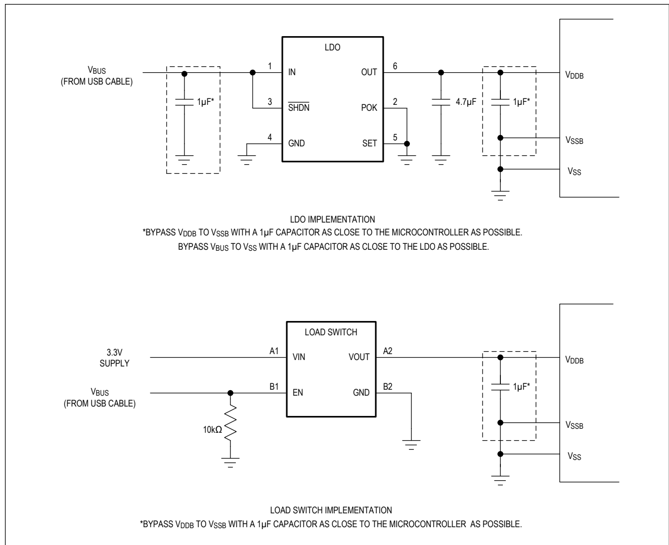
Figure 9. V DDB Signal Implementation, 140-Bump WLP
