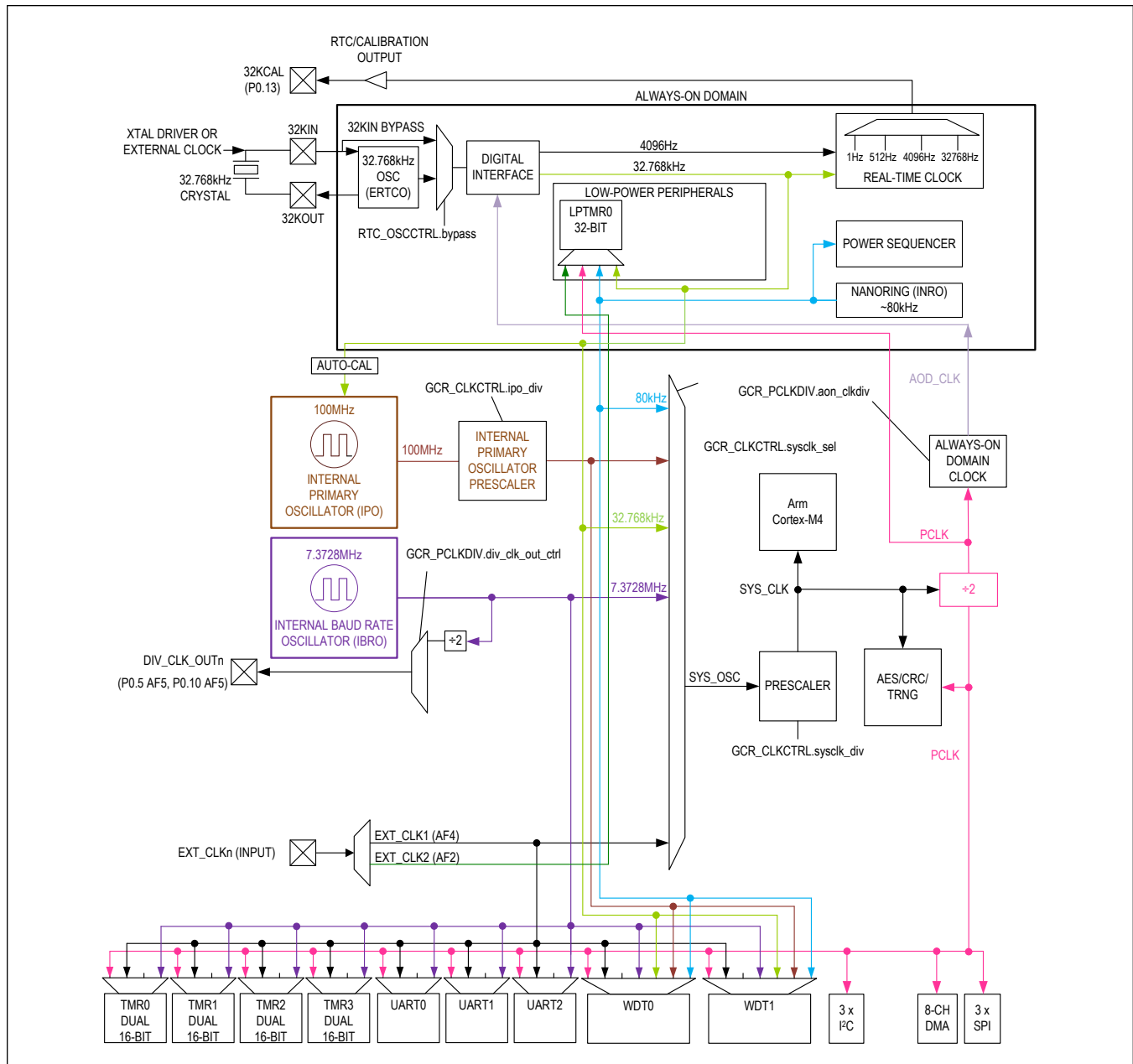
Figure 9. 24 WLP Clocking Scheme
