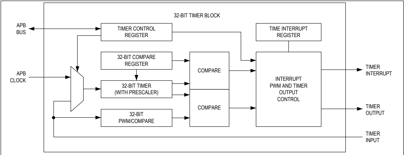
Figure 7. 32-Bit Timer
