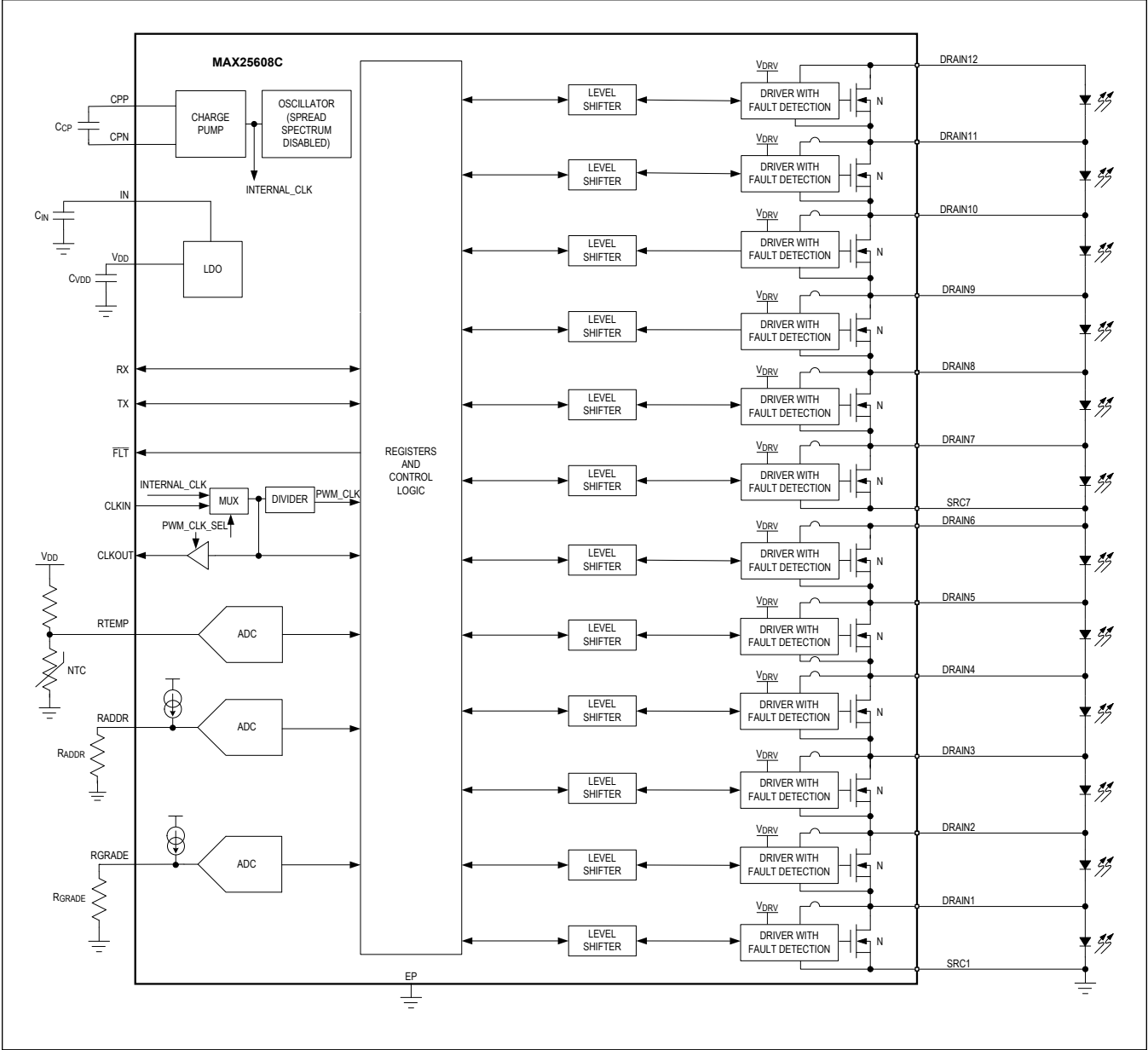
MAX25608C Block Diagram
