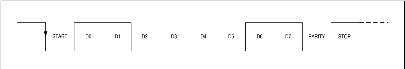
Figure 12. ACK Frame
