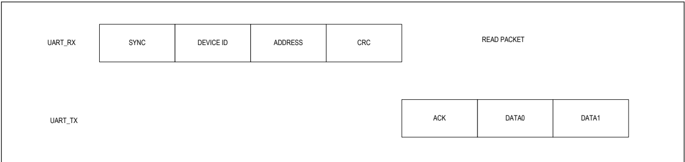
Figure 15. Read Packet
