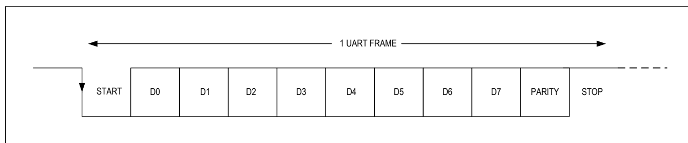
Figure 8. Frame Format
