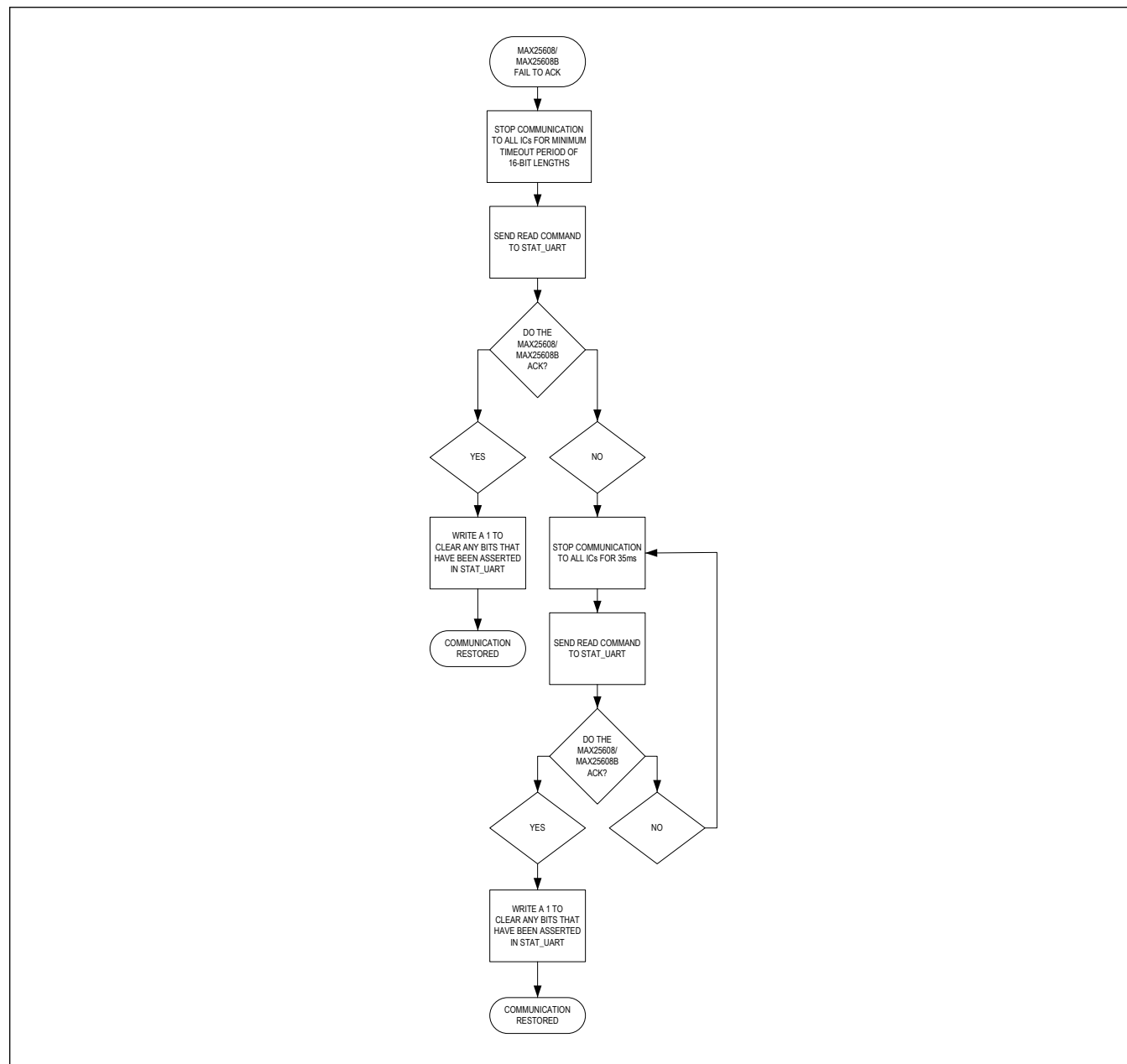
Figure 17. Timeout Flowchart
