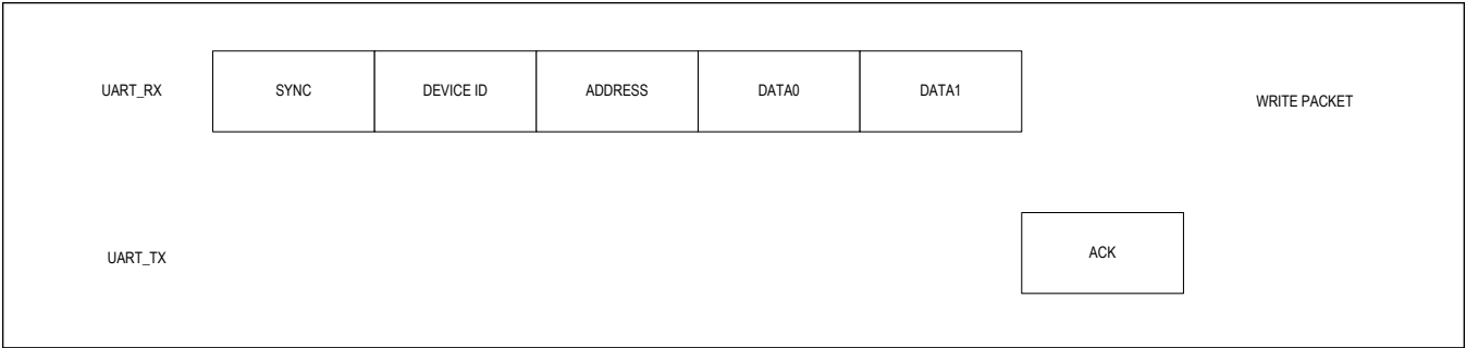
Figure 14. Write Packet
