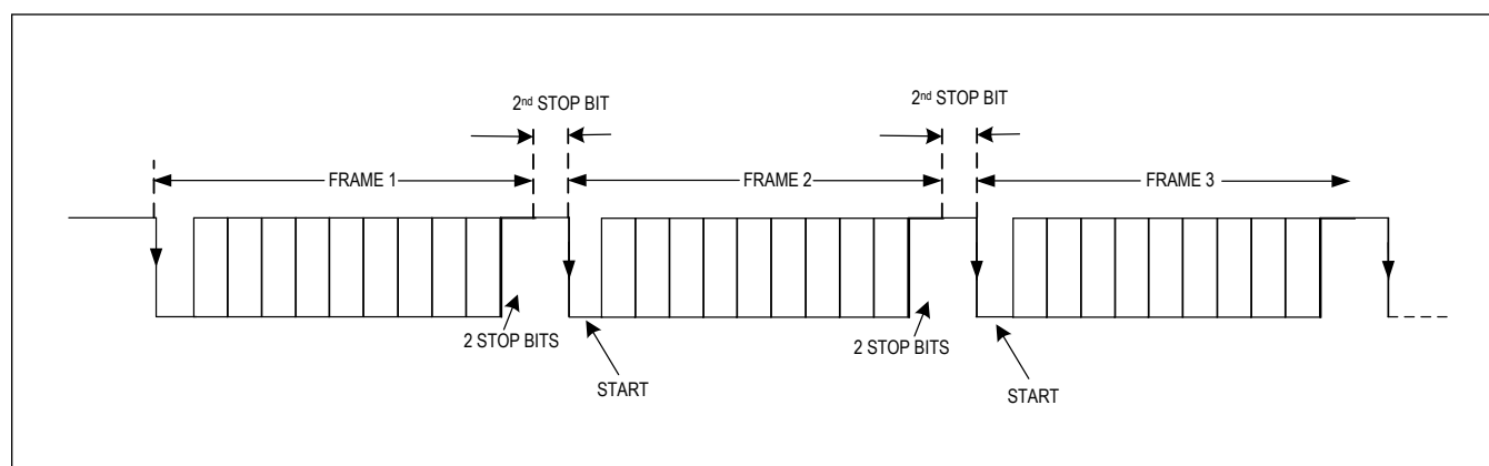
Figure 9. Interframe Format
