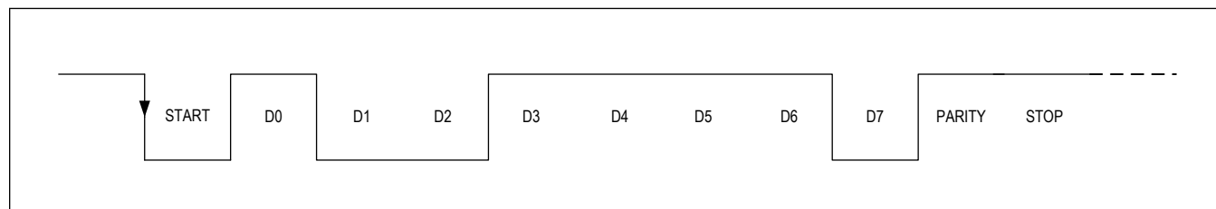
Figure 11. SYNC Frame
