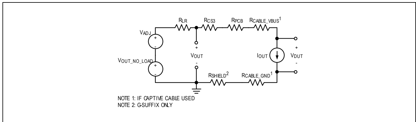
Figure 38. DC Voltage Adjustment Model
