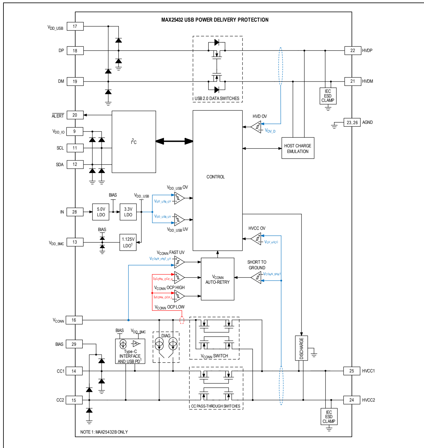
Figure 15. USB Power Delivery Protection Block Diagram
