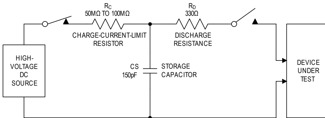
Figure 46. IEC 61000-4-2 ESD Test Model
