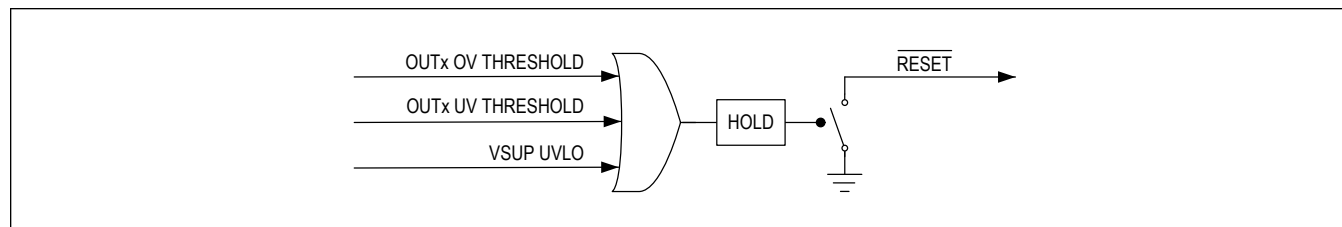
Figure 2. Simplified RESET Logic Diagram
