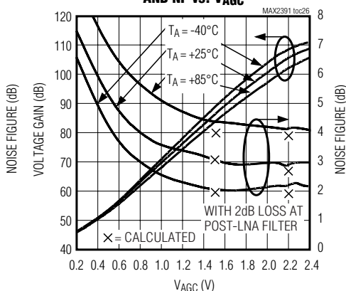
CASCADE GAIN (HGML MODE) AND NF vs. V_{AGC}
