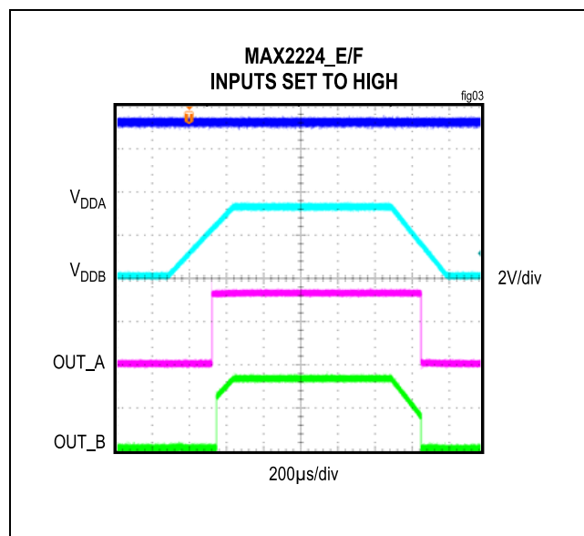
Figure 3. Undervoltage Lockout Behavior MAX2224_E/F Input High
