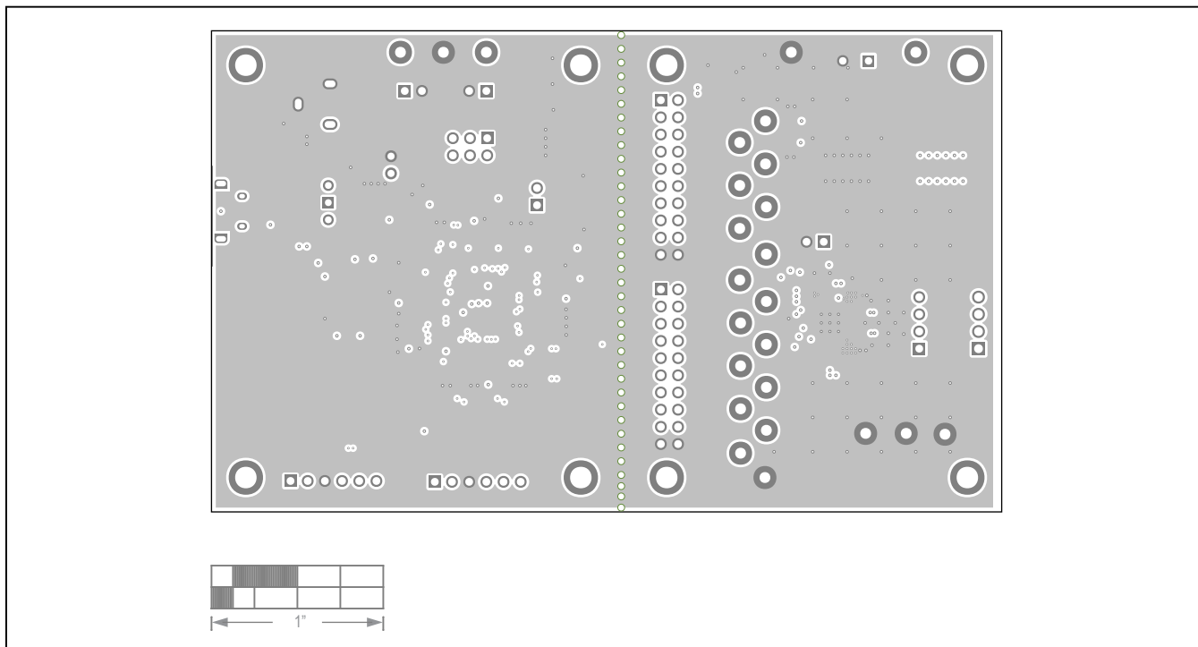
MAX22210 EV Kit PCB Layout—GND Plane
