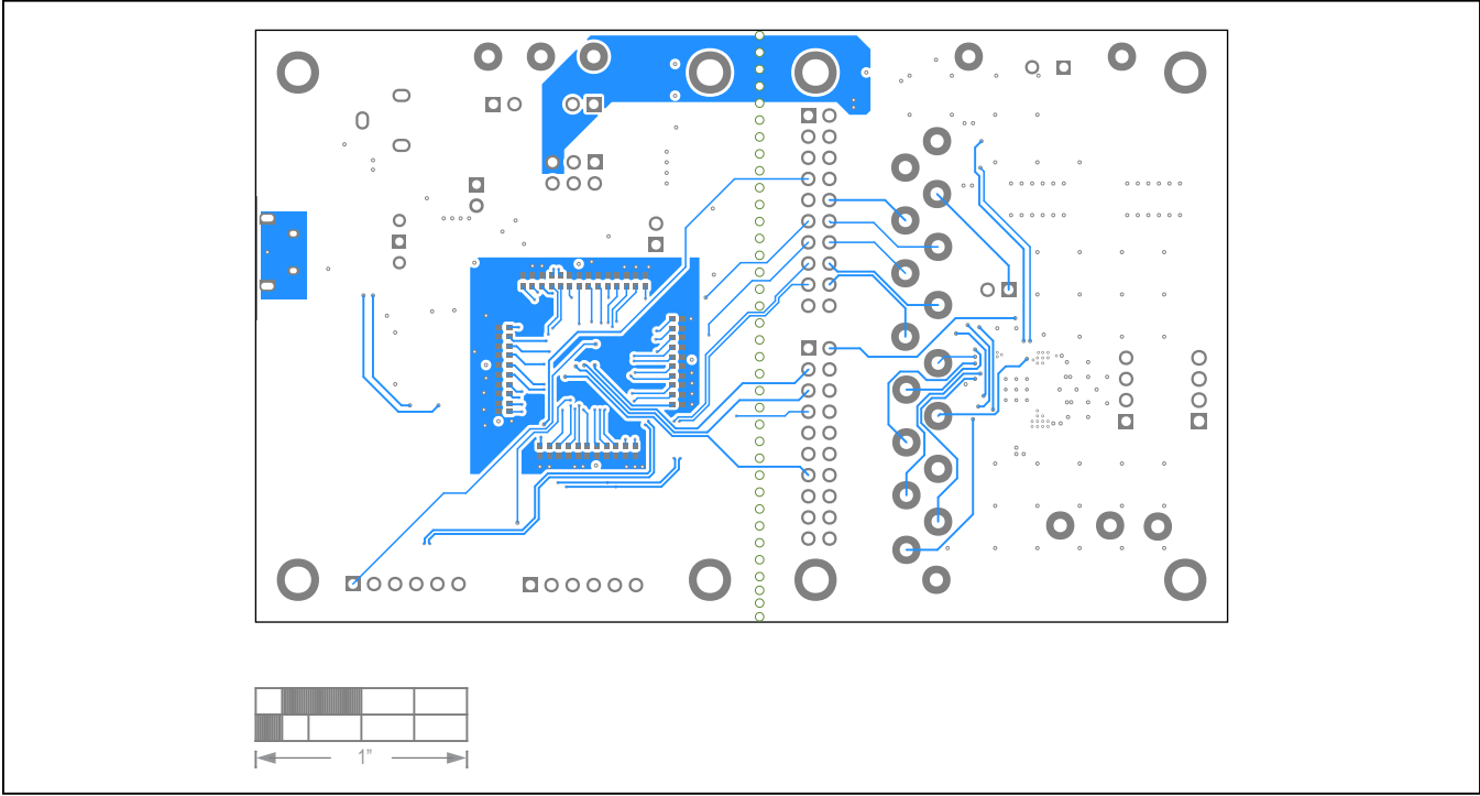
MAX22210 EV Kit PCB Layout—Bottom Layer
