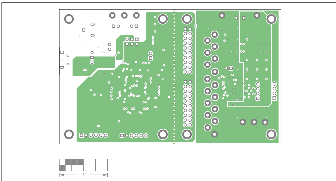
MAX22210 EV Kit PCB Layout—Power Plane
