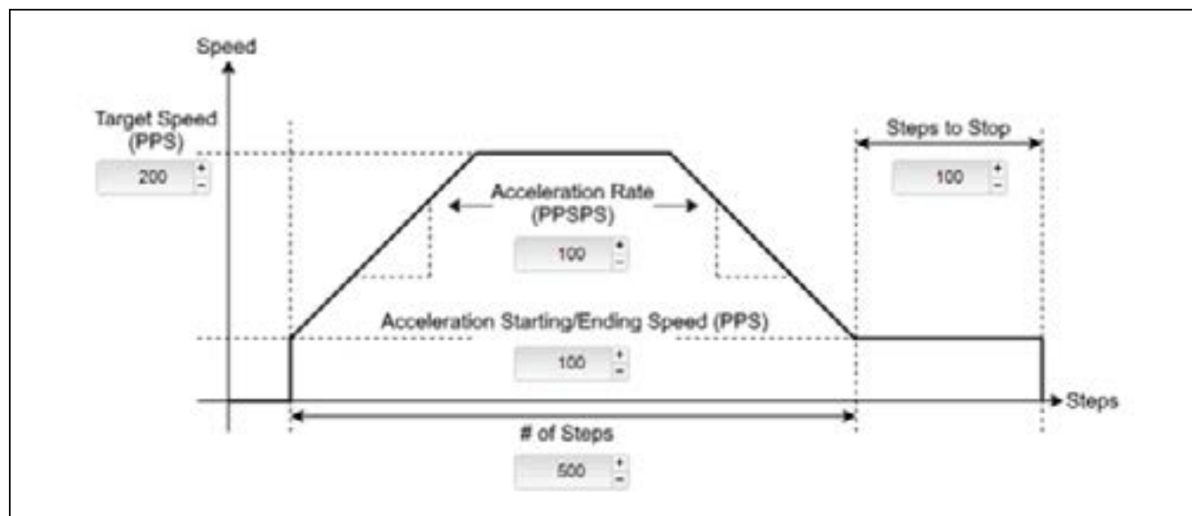
Figure 5. Motor-Control Graph
