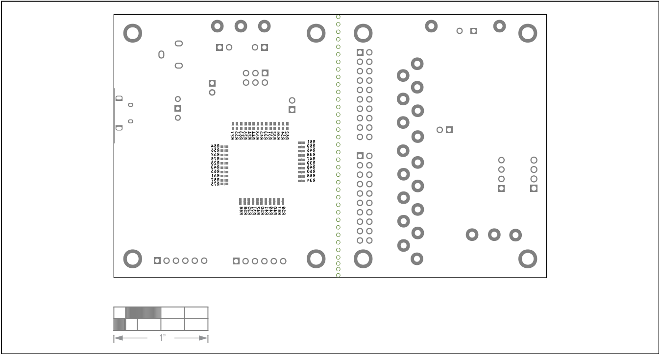
MAX22210 EV Kit PCB Layout—Bottom Silkscreen
