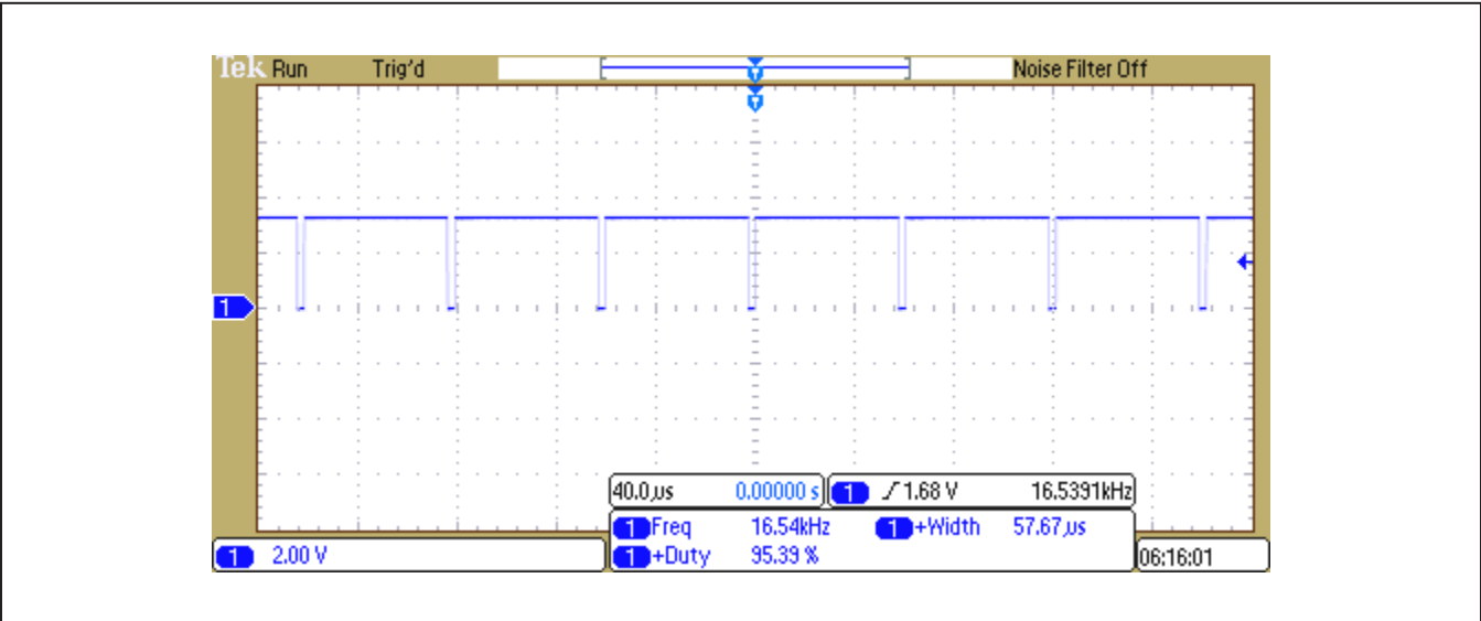
Figure 4. PWM Signal Measured at Test Point TP3 with a 95% Duty Cycle
