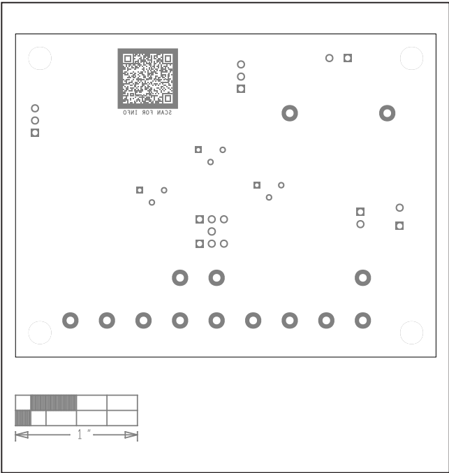
MAX22202 EV Kit Component Placement Guide—Bottom Silkscreen
