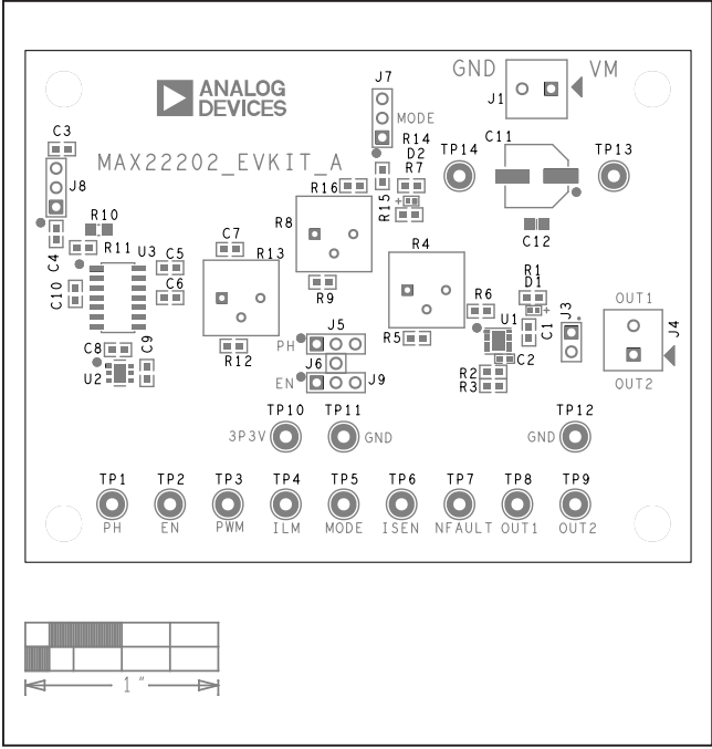
MAX22202 EV Kit Component Placement Guide—Top Silkscreen
