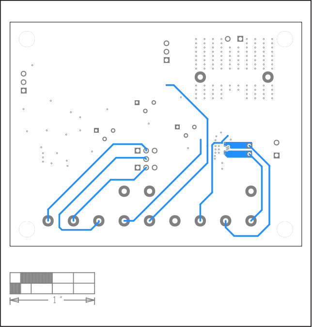
MAX22202 EV Kit PCB Layout—Bottom
