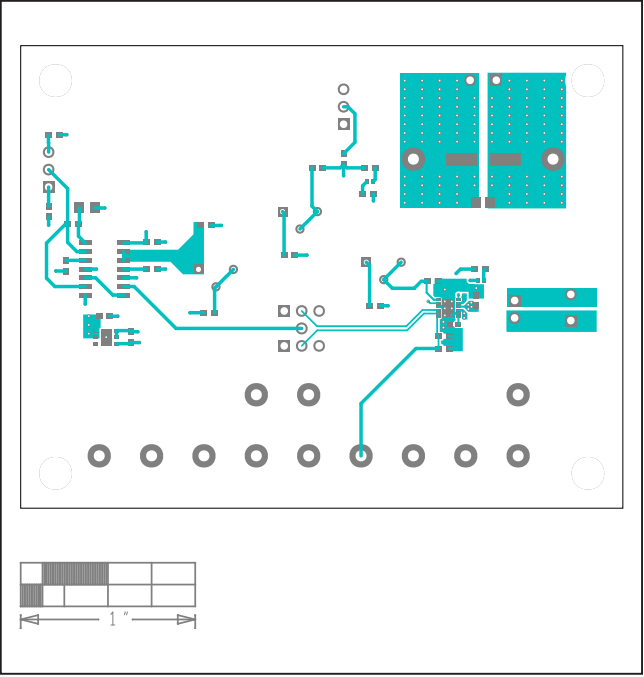
MAX22202 EV Kit PCB Layout—Top
