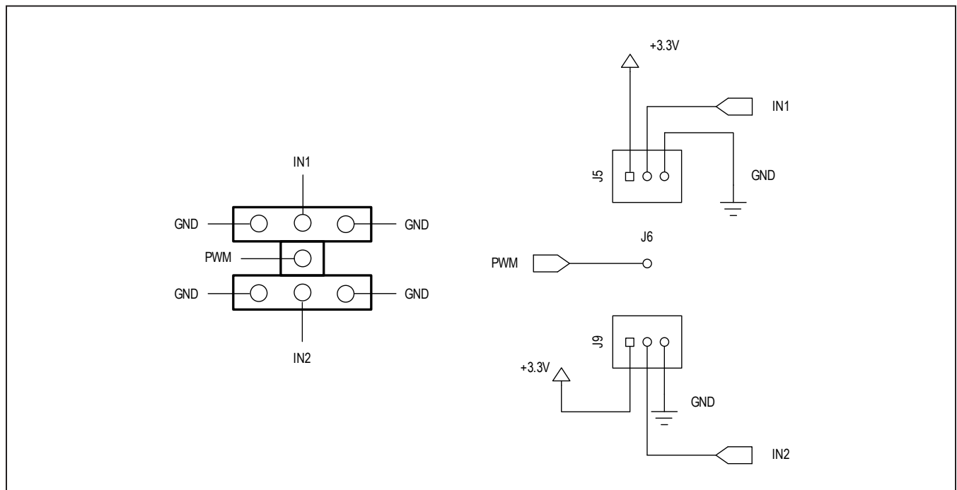
Figure 2. Configuration of the MAX22202 Input Headers J5, J6, and J9
