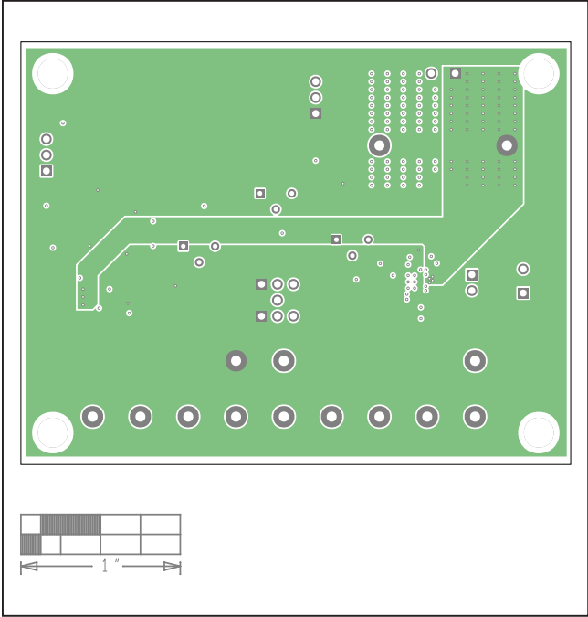
MAX22202 EV Kit PCB Layout—Internal3
