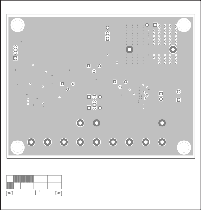
MAX22202 EV Kit PCB Layout—Internal2
