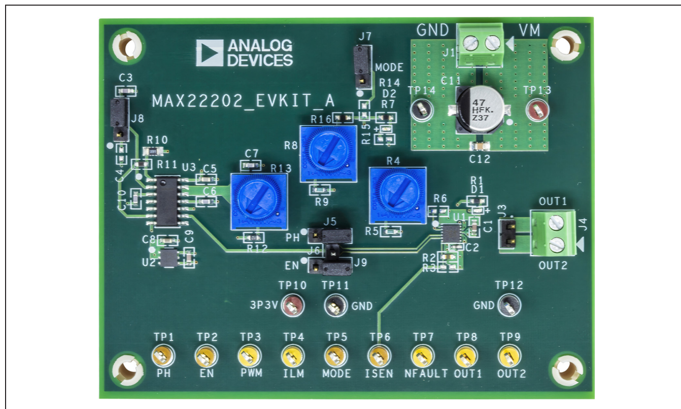
Figure 1. MAX22202 EV Kit Board
