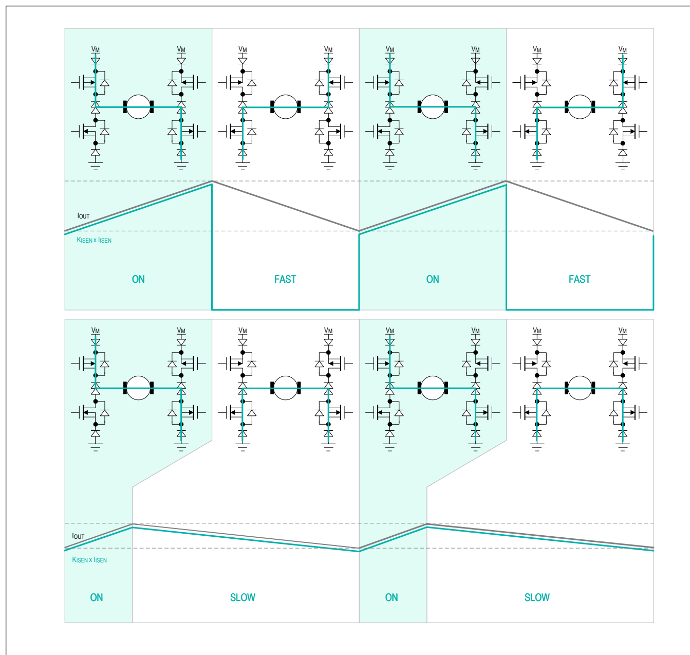
Figure 1. ISEN Current
