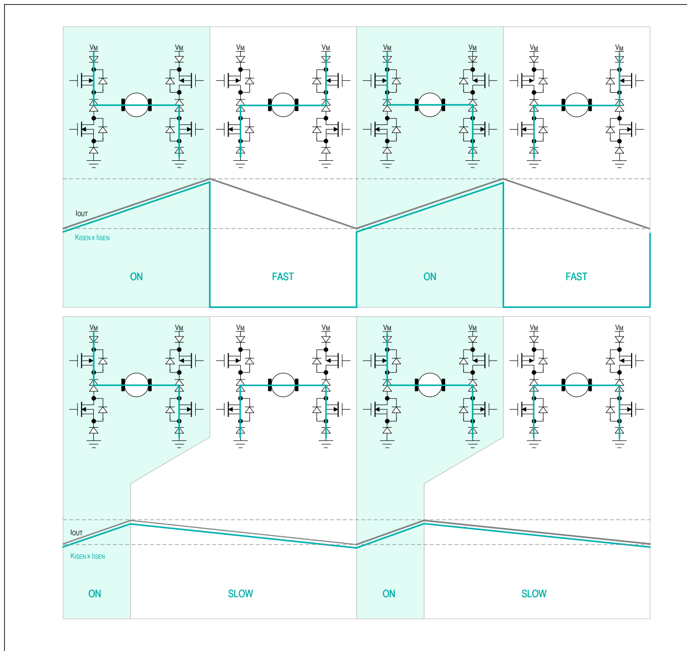
Figure 1. ISEN Current
