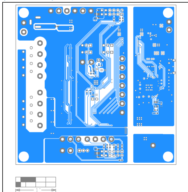
MAX22196 EV Kit PCB Layout—Bottom
