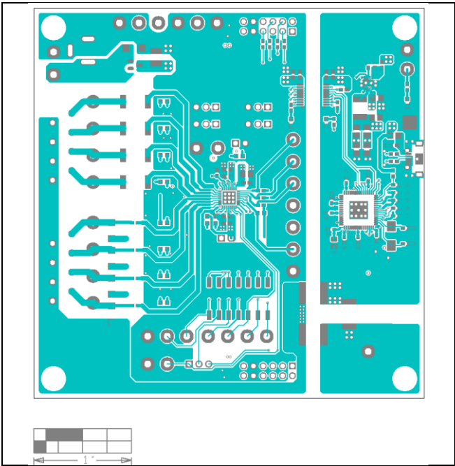
MAX22196 EV Kit PCB Layout—Top
