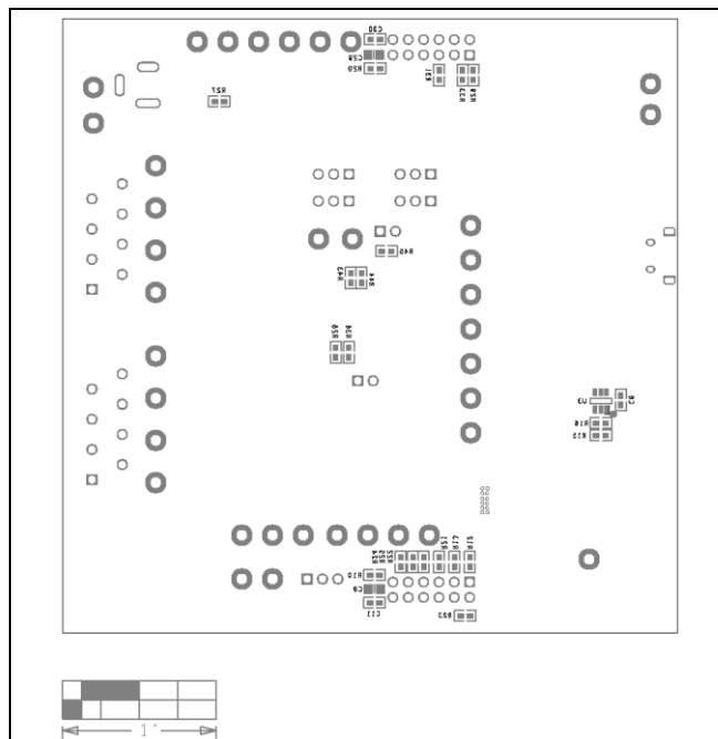
MAX22196 EV Kit Component Placement Guide—Bottom Silkscreen
