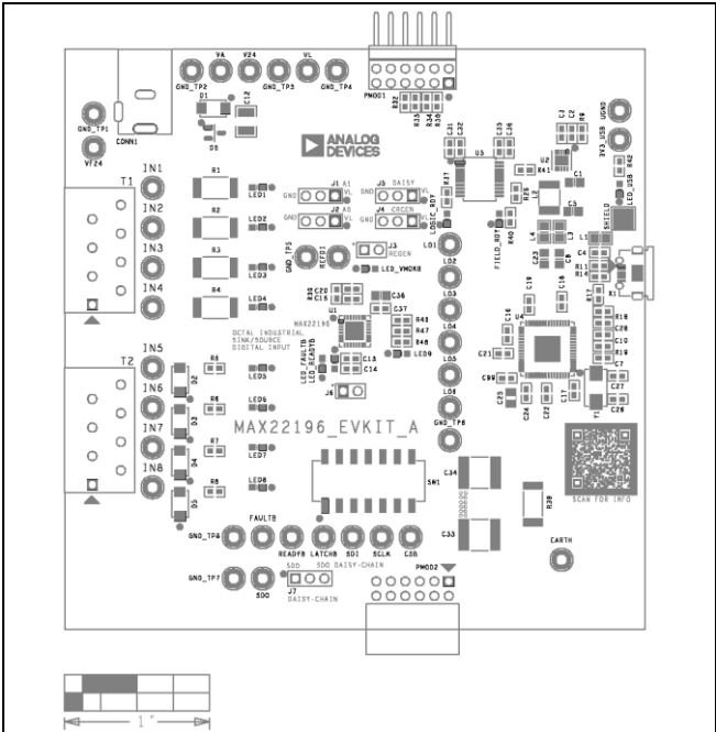
MAX22196 EV Kit Component Placement Guide—Top Silkscreen
