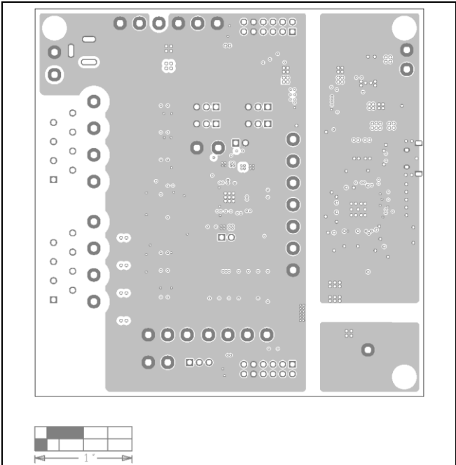
MAX22196 EV Kit PCB Layout—Layer 2
