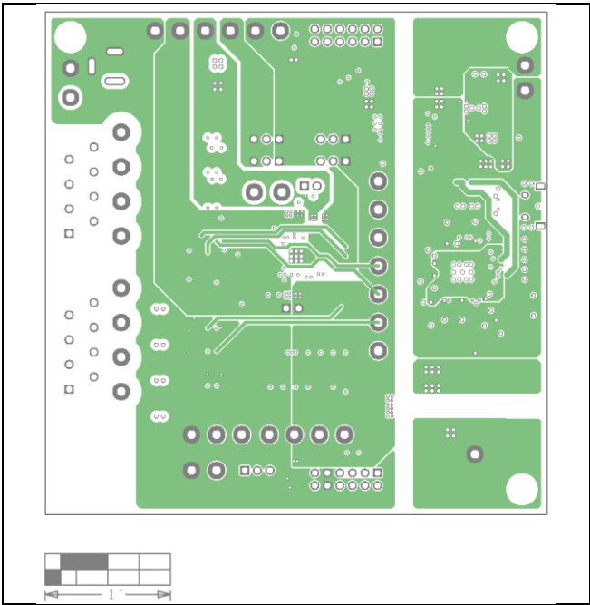
MAX22196 EV Kit PCB Layout—Layer 3
