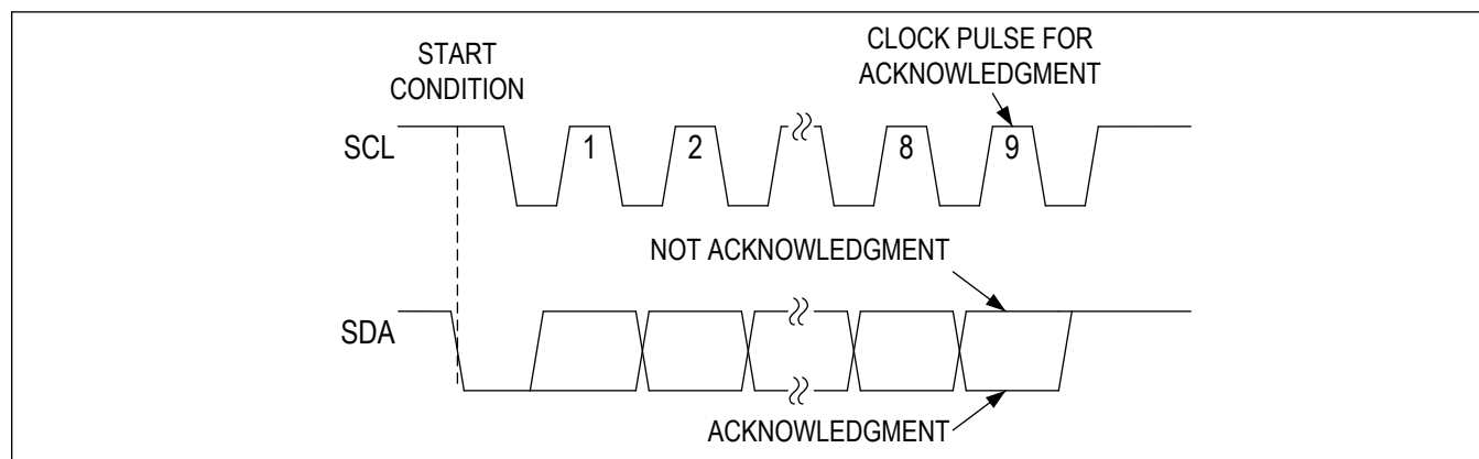
Figure 2. Acknowledge Condition
