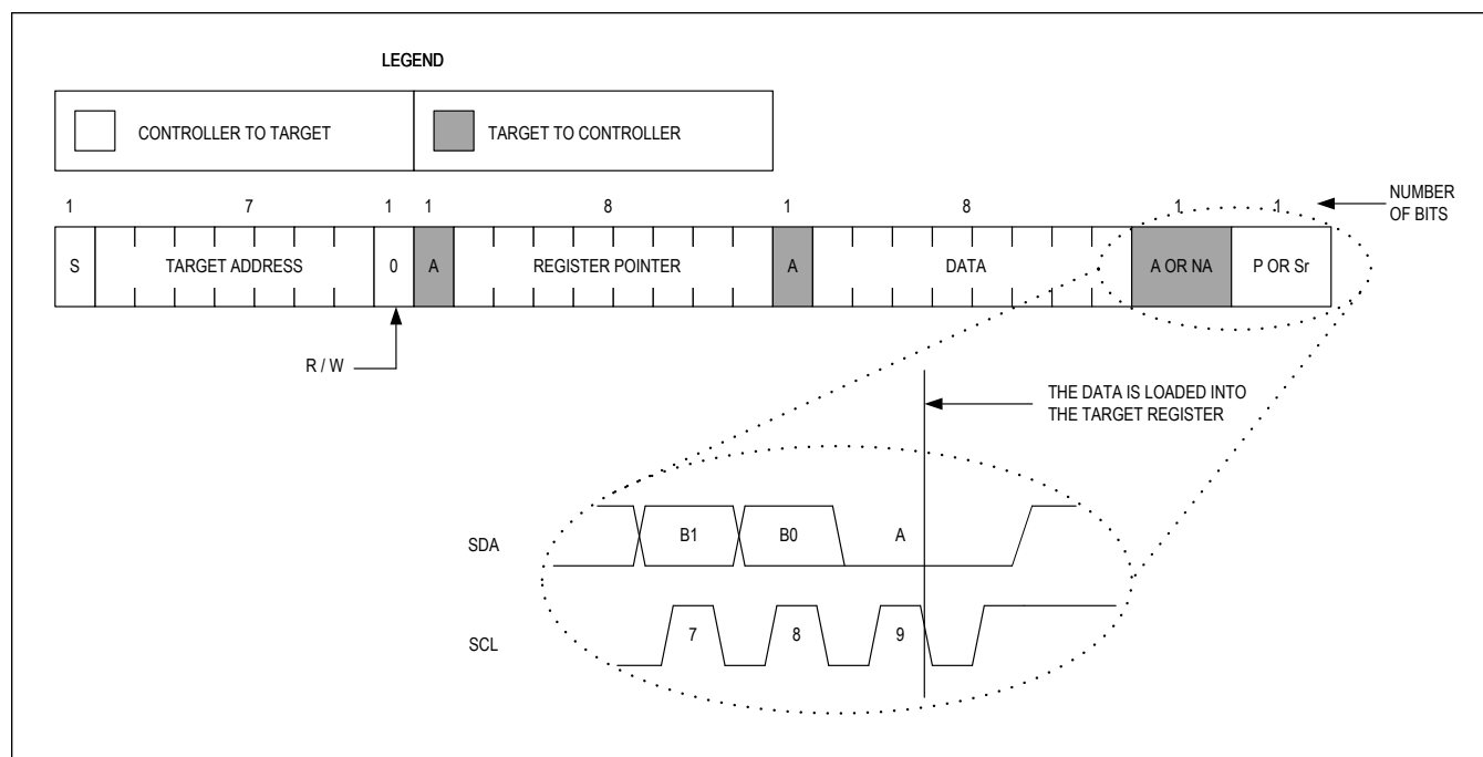
Figure 4. Write-Byte Format
