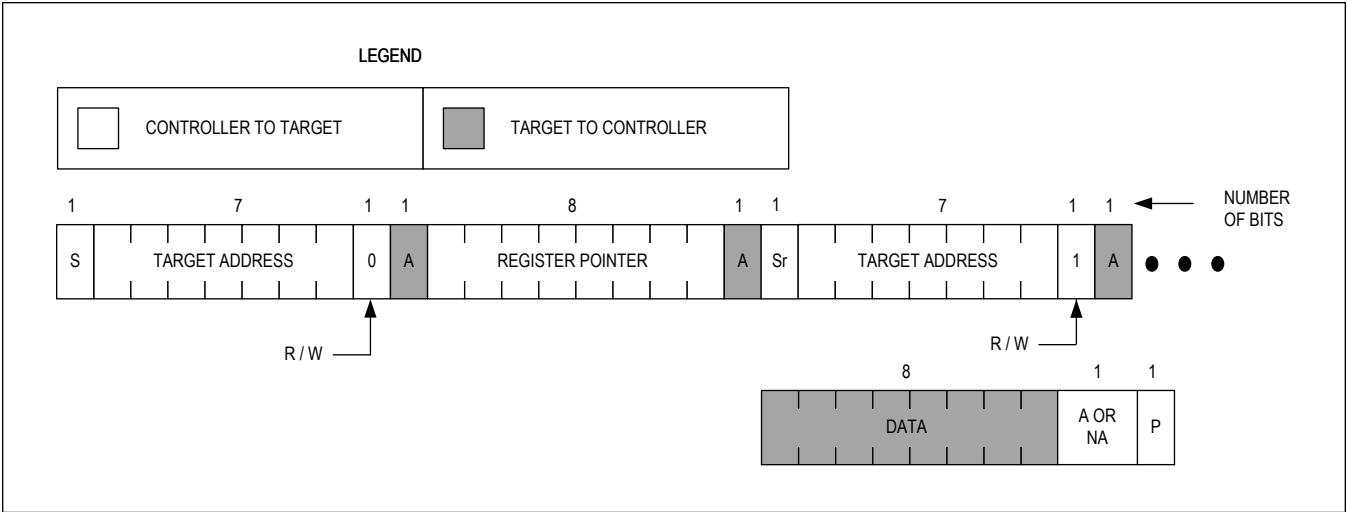
Figure 6. Read-Byte Format
