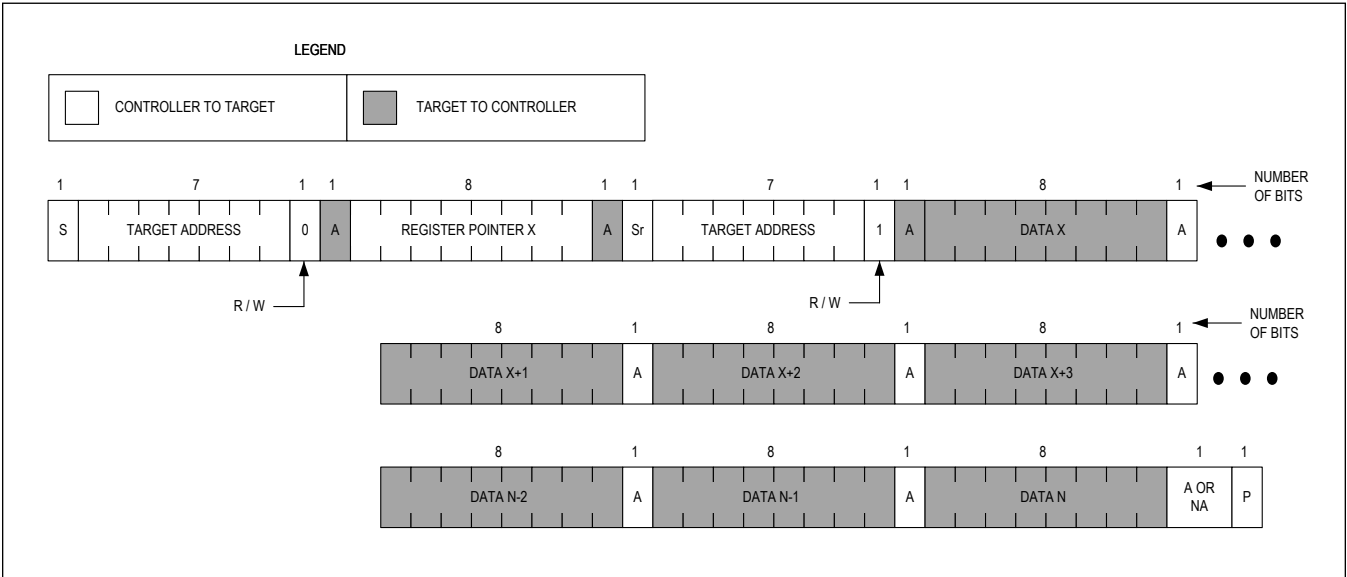
Figure 7. Sequential-Read Format
