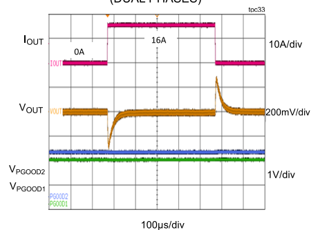
LOAD TRANSIENT RESPONSE (DUAL PHASES)
