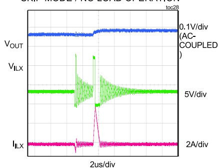
SKIP MODE / NO LOAD OPERATION
