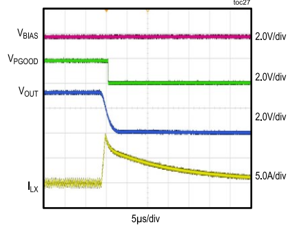
SHORT-CIRCUIT RESPONSE (MAX20406AFOB)
