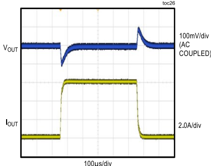
LOAD TRANSIENT (MAX20406AFOB, C_{OUT} = 42\mu F EFFECTIVE)
