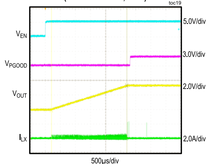
STARTUP INTO NO LOAD (MAX20406AFOB, SKIP)
