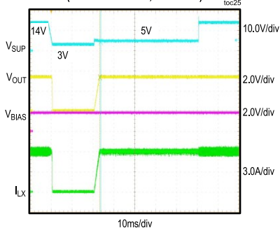
COLD CRANK (MAX20406AFOB, 6A LOAD)
