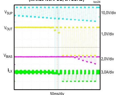
DIPS AND DROPS (MAX20406AFOB, 3A LOAD)
