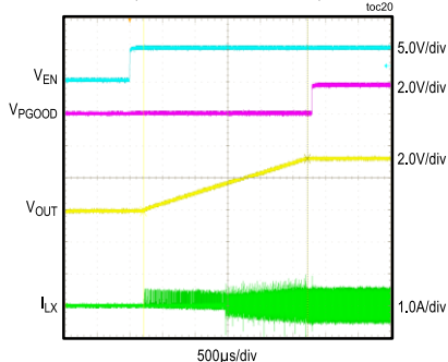
STARTUP INTO NO LOAD (MAX20406AFOB, FPWM)
