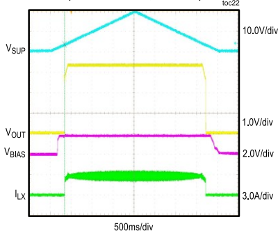
SLOW INPUT VOLTAGE RISING (MAX20406AFOB, 3A LOAD)
