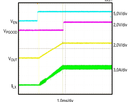
STARTUP INTO FULL LOAD (MAX20406AFOB, FPWM)
