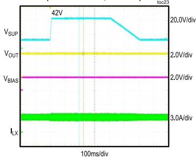
LOAD DUMP (MAX20406AFOB, 3A LOAD)
