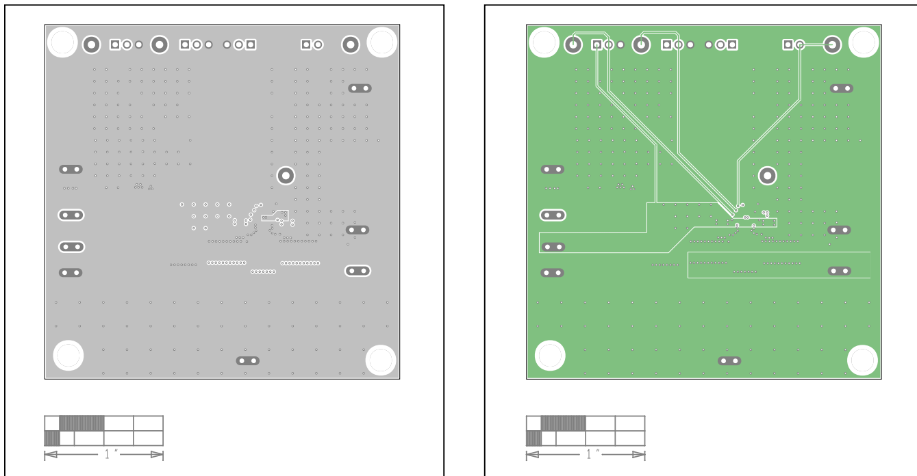
MAX20403 Evaluation Kit Layout—Internal Layers Are Ground Planes
