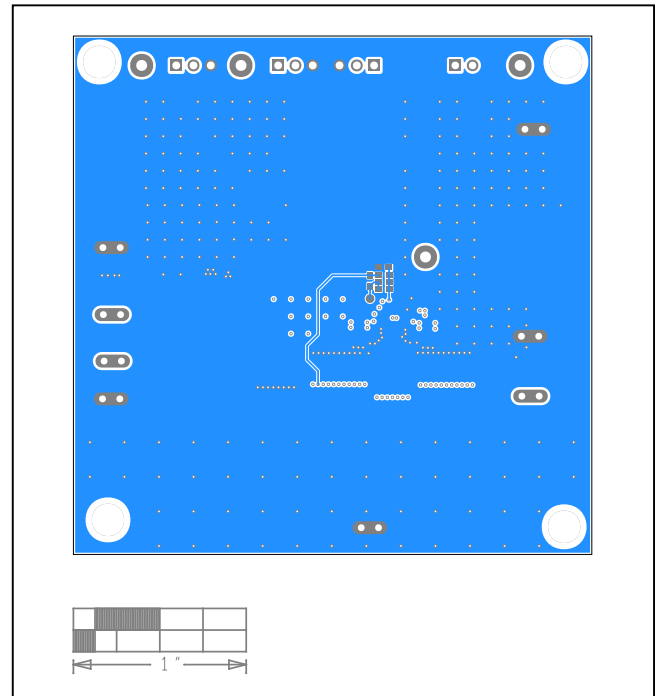
MAX20403 Evaluation Kit Layout—Bottom Layer
