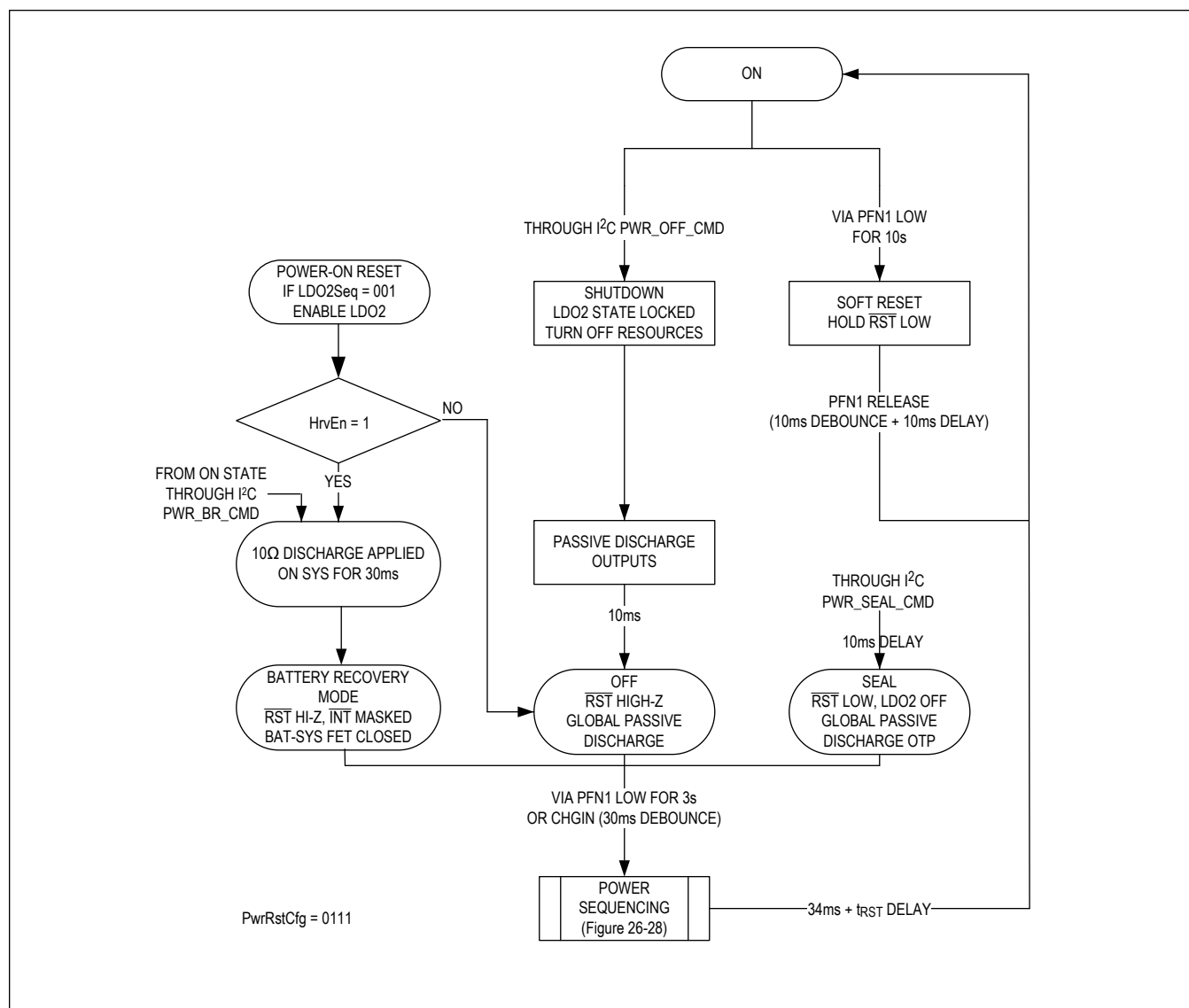
Figure 19. PwrRstCfg 0111
