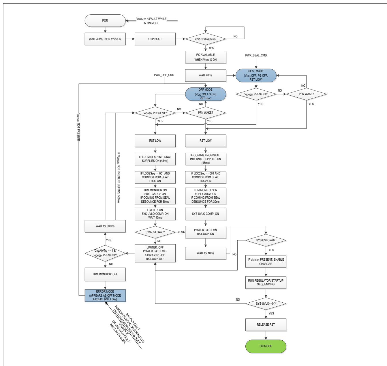
Figure 24. Boot Sequence—Harvester Mode Disabled
