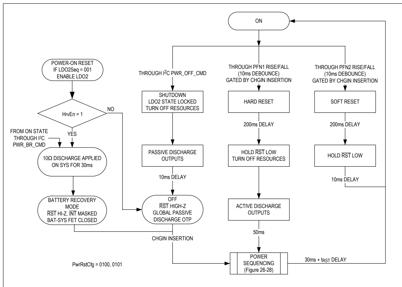
Figure 17. PwrRstCfg 0100, 0101
