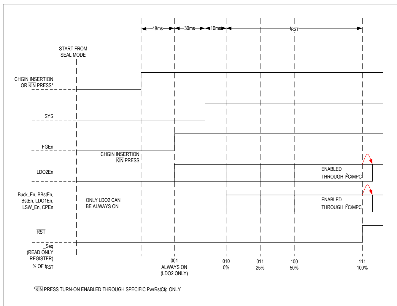
Figure 28. Power Sequencing, from SEAL Mode
