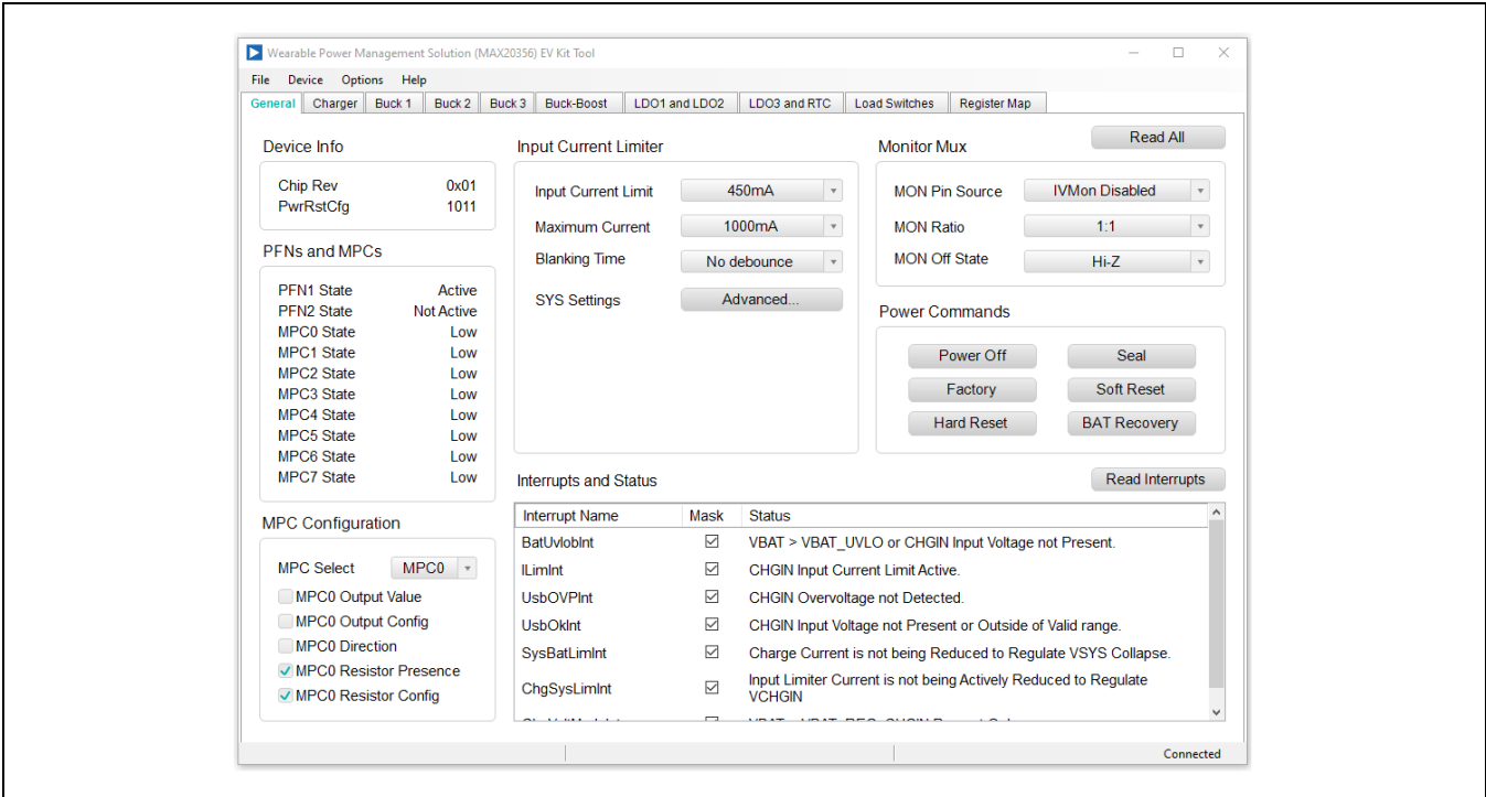
Figure 2. Connected Status
