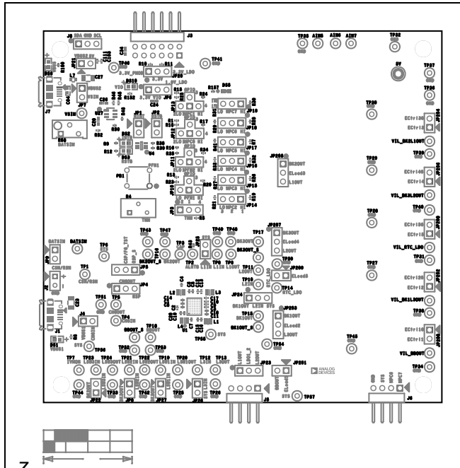
MAX20356 EV Kit Component Placement Guide—Top Silkscreen
