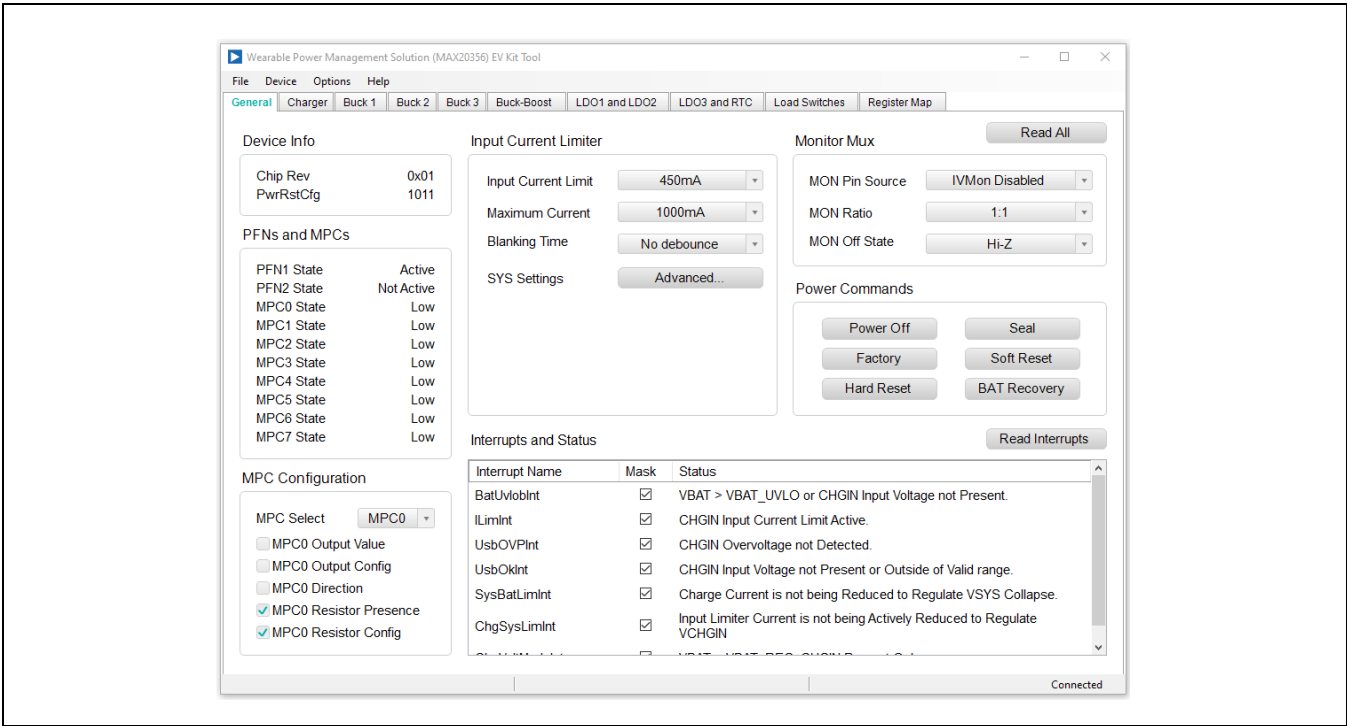
Figure 4. General Tab
