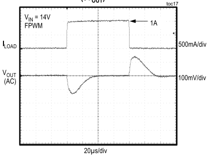
LOAD-TRANSIENT RESPONSE (5V OUT )
