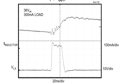
MINIMUM ON-TIME (1.8V OUT )
