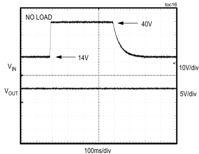
LOAD-DUMP TEST
