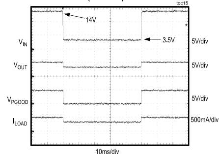
UNDERVOLTAGE PULSE (NO LOAD)
