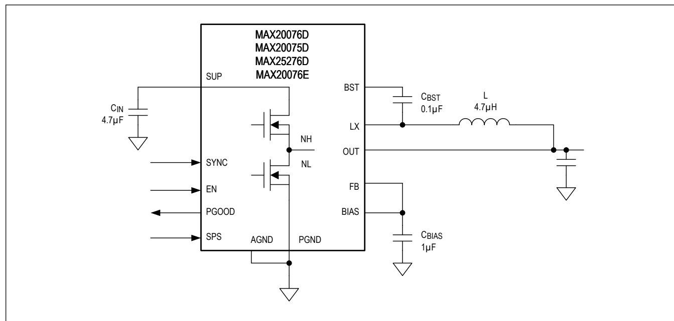
Figure 2. MAX20075D/MAX20076D/MAX20076E/MAX25276D Application Circuit with Fixed Output Voltage
