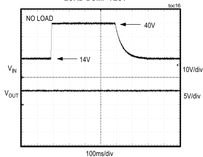
LOAD-DUMP TEST
