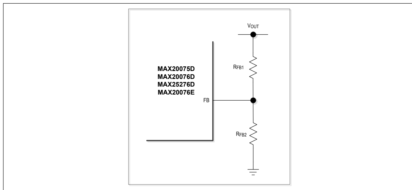
Figure 1. Connecting a Resistive Divider from Output to FB to AGND
