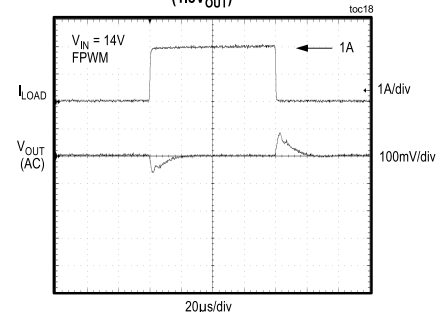
LOAD-TRANSIENT RESPONSE (1.8V OUT )
