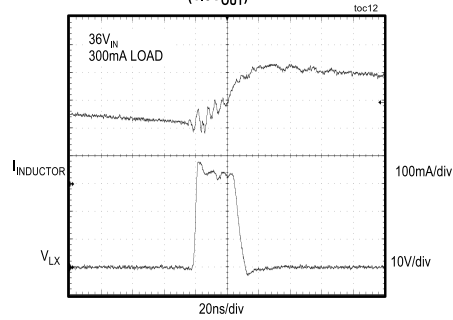
MINIMUM ON-TIME (1.8V OUT )
