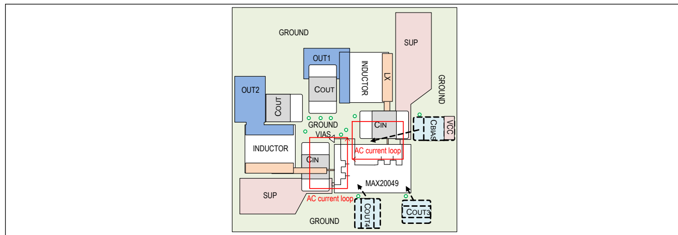
Figure 5. MAX20049 PCB Layout
