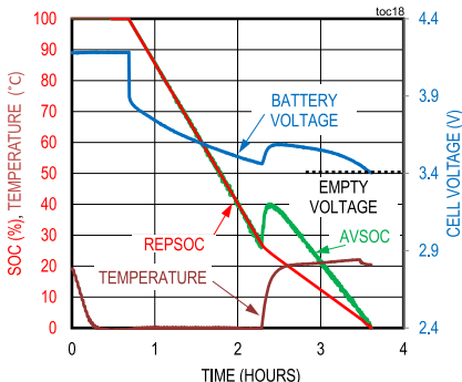
RESPONSE TO TEMPERATURE TRANSIENT AT CONSTANT-CURRENT LOAD
