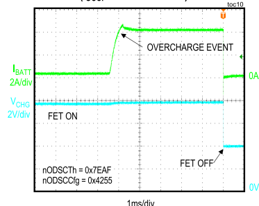
OVERCHARGE CURRENT PROTECTION ( I_{OCP} = 4\text{A}/5\text{ms DELAY} )
