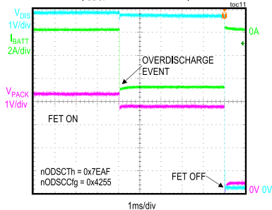
OVERDISCHARGE CURRENT PROTECTION ( I_{OCP} = 4\text{A}/5\text{ms DELAY} )
