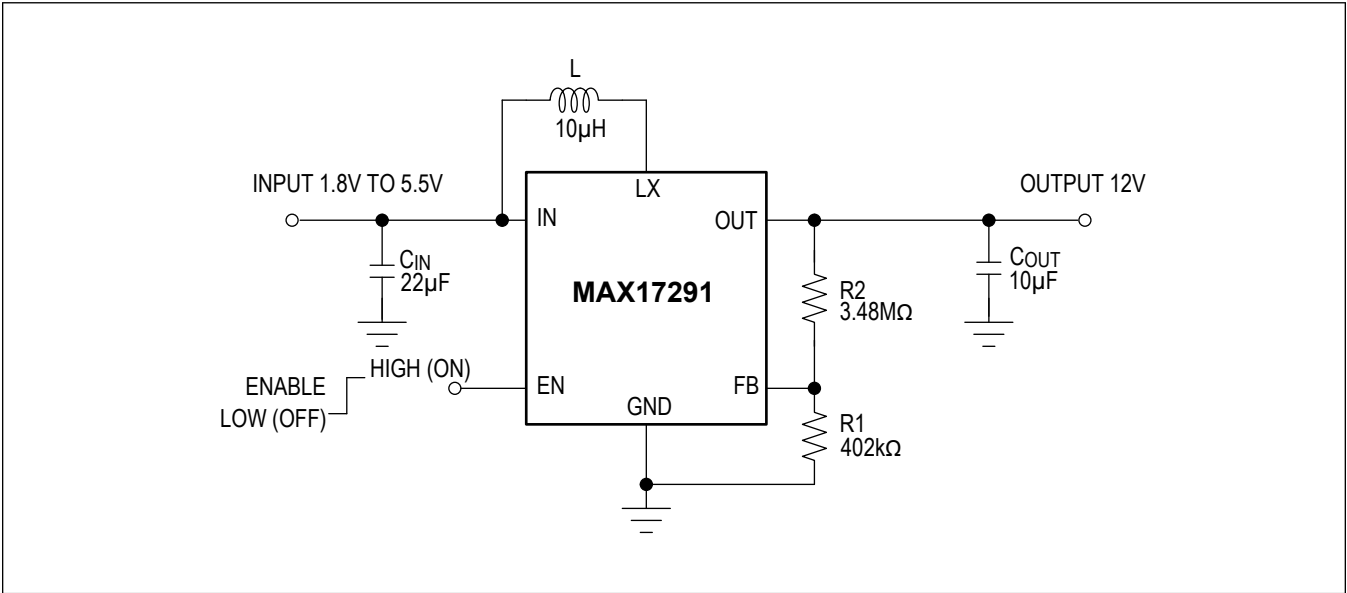
Figure 2. 12V Boost Converter Using the MAX17291
