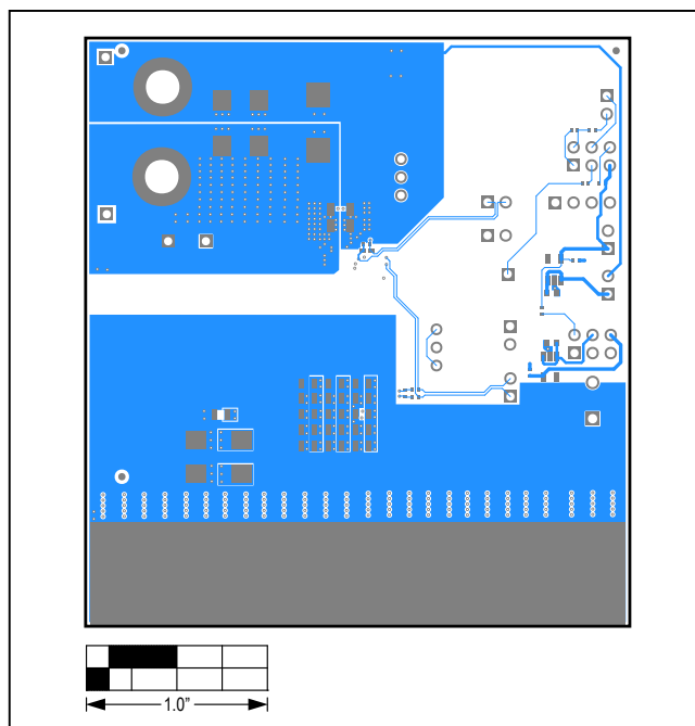
MAX16425/MAX16425A PCB Layout—Bottom View
