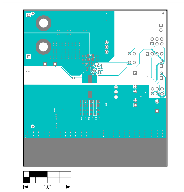
MAX16425/MAX16425A PCB Layout—Top View
