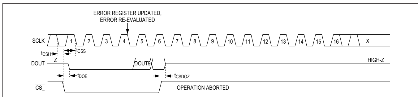
Figure 10. Aborted SPI Programming Operation (Invalid, Showing t_{\text{CSPOZ}} and Internal Activity)
