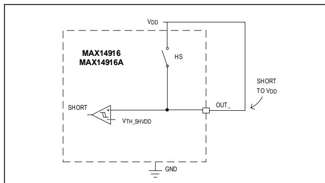
Figure 6. Short-to- V_{DD} Detection Scheme
