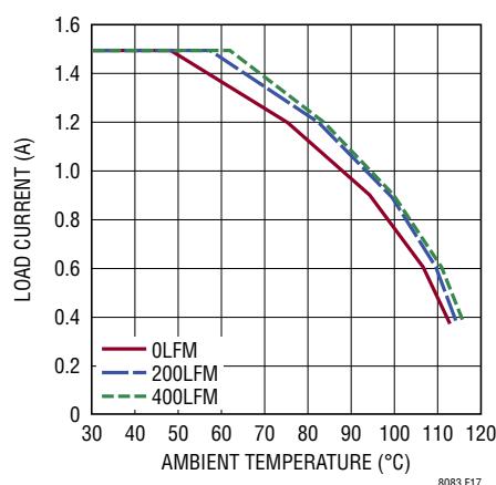
Figure 17. 12V to 12V Derating Curve, No Heat Sink
