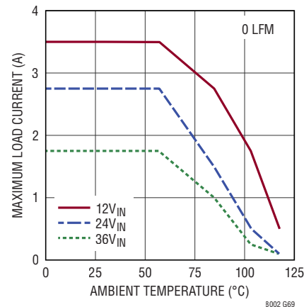
Derating, I-Grade, V_{OUT} = 8\text{V} , BIAS = 5V, DC2501A Demo Board
