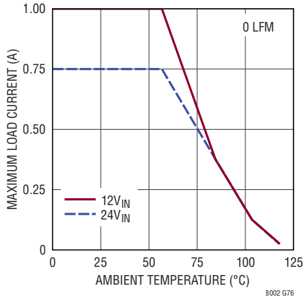
Derating, I-Grade, V_{OUT} = -12\text{V} , BIAS Tied to LTM8002 GND, DC2501A Demo Board
