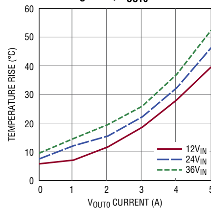
Temperature Rise vs V_{OUT0} Current, Buck Regulator, V_{OUT0} = 2.5\text{V}
