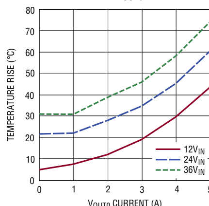
Temperature Rise vs V_{OUT0} Current, Buck Regulator, V_{OUT0} = 8\text{V}
