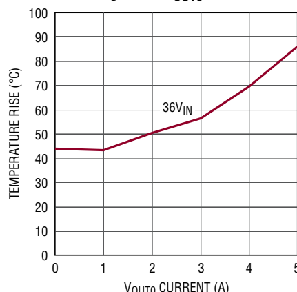
Temperature Rise vs V_{OUT0} Current, Buck Regulator, V_{OUT0} = 24\text{V}
