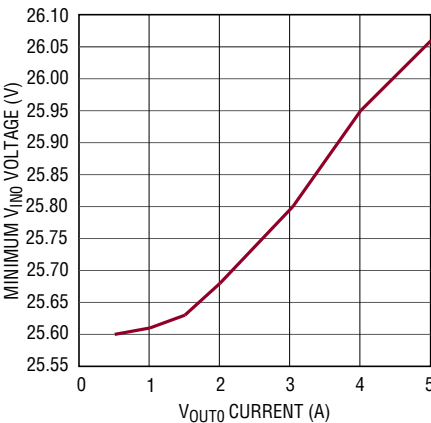
Minimum V_{IN0} vs Output Current, V_{OUT0} = 24\text{V}
