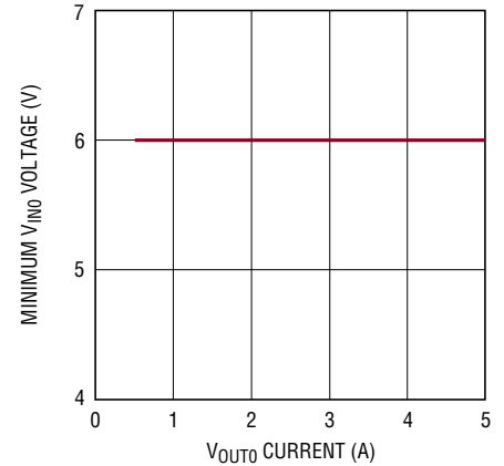
Minimum V_{IN0} vs Output Current, V_{OUT0} = 3.3\text{V} and Below
