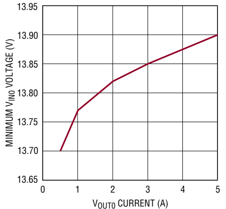
Minimum V_{IN0} vs Output Current, V_{OUT0} = 12\text{V}
