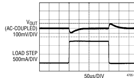
3.3V Output Transient Response
