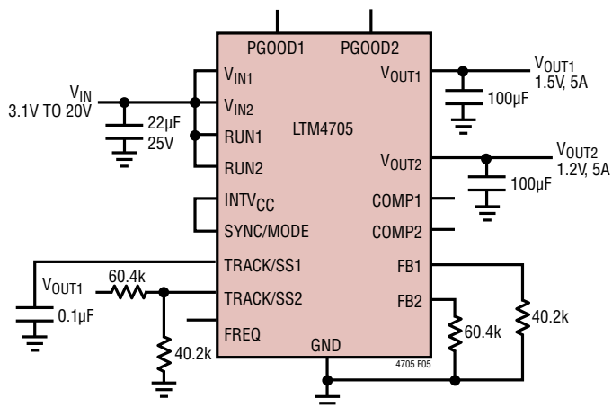
Figure 5. Example Schematic of Ratiometric Output Voltage Tracking
