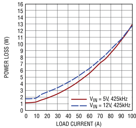
Figure 37. 1.2V Power Loss Curve
