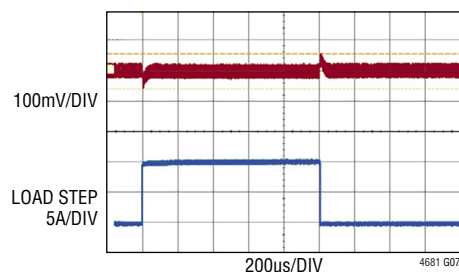
Single Channel Load Transient Response (10A) to (20A) Load Step, 10\text{A}/\mu\text{s} 12\text{V}_{\text{IN}} , \text{V}_{\text{OUT}} = 1.5\text{V} , f_{\text{SW}} = 350\text{kHz}
