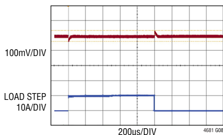
Single Channel Load Transient Response (10A) to (20A) Load Step, 10\text{A}/\mu\text{s} 12\text{V}_{\text{IN}} , \text{V}_{\text{OUT}} = 2.5\text{V} , f_{\text{SW}} = 500\text{kHz}
