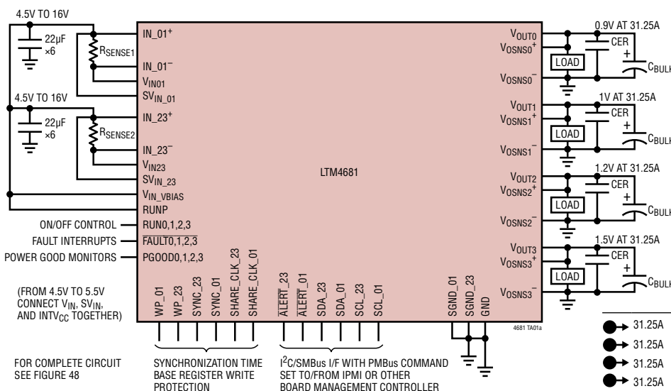
Configurable Output Array
