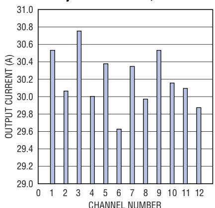
READ_IOUT of 12 LTM4681 Channels 12\text{V}_{\text{IN}} , 1\text{V}_{\text{OUT}} , T_J = 25^\circ\text{C} , I_{\text{OUT}n} = 30\text{A} , System Having Reached Thermally Steady-State Condition, No Airflow
