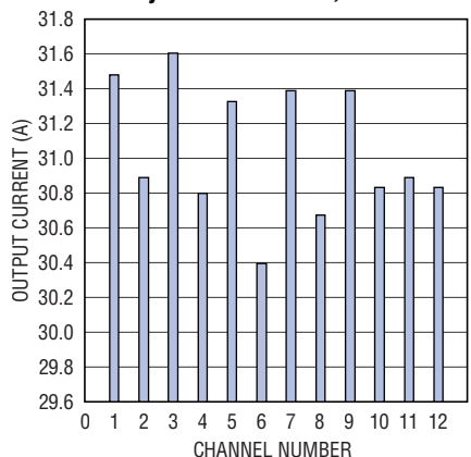
READ_IOUT of 12 LTM4681 Channels 12\text{V}_{\text{IN}} , 1\text{V}_{\text{OUT}} , T_J = -40^\circ\text{C} , I_{\text{OUT}n} = 30\text{A} , System Having Reached Thermally Steady-State Condition, No Airflow
