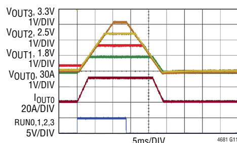
FIGURE 48 CIRCUIT, 12\text{V}_{\text{IN}} , 30\text{A} ON \text{V}_{\text{OUT0}} NO LOAD ON OTHER OUTPUTS AND 0.5\text{V} PREBIAS ON \text{V}_{\text{OUT1}}
