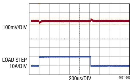
Single Channel Load Transient Response (10A) to (20A) Load Step, 10\text{A}/\mu\text{s} 12\text{V}_{\text{IN}} , \text{V}_{\text{OUT}} = 1.2\text{V} , f_{\text{SW}} = 350\text{kHz}
