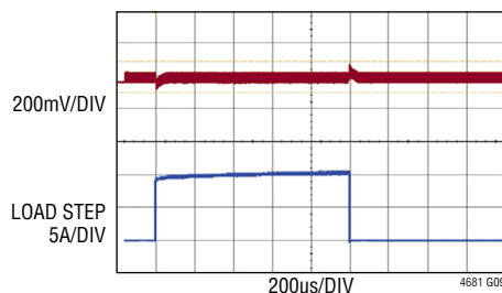
Single Channel Load Transient Response (10A) to (20A) Load Step, 10\text{A}/\mu\text{s} 12\text{V}_{\text{IN}} , \text{V}_{\text{OUT}} = 3.3\text{V} , f_{\text{SW}} = 500\text{kHz}
