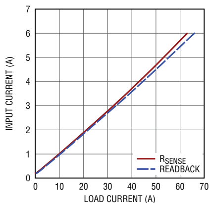
Supply Current vs Load Current Comparison, R_{\text{SENSE}} = 2\text{m}\Omega , 12\text{V} to 1.0\text{V}_{\text{OUT}} , 250\text{kHz}
