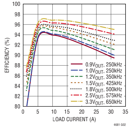
Single Channel Efficiency, 8V_{IN} , V_{IN} = SV_{IN} = V_{IN\_VBIAS} = 8V , RUNP = 8V , CCM Mode
