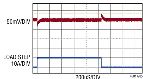
Single Channel Load Transient Response (10A) to (20A) Load Step, 10\text{A}/\mu\text{s} 12\text{V}_{\text{IN}} to 0.9\text{V}_{\text{OUT}}
