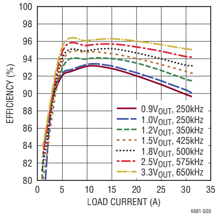
Single Channel Efficiency, 12V_{IN} , V_{IN} = SV_{IN} = V_{IN\_VBIAS} = RUNP = 12V , CCM Mode
