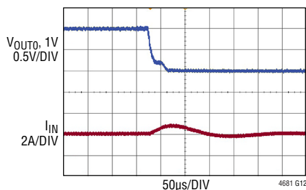
FIGURE 48 CIRCUIT, 12\text{V}_{\text{IN}} , NO LOAD ON \text{V}_{\text{OUT0}} PRIOR TO APPLICATION OF SHORT-CIRCUIT USE HIGH RANGE OF \text{I} LIMIT SYSTEM SHORT-CIRCUIT USING LOW IMPEDANCE COPPER ACROSS OUTPUT (HARD SHORT)
