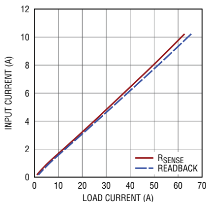
Supply Current vs Load Current Comparison, R_{\text{SENSE}} = 2\text{m}\Omega , 12\text{V} to 1.8\text{V}_{\text{OUT}} , 500\text{kHz}
