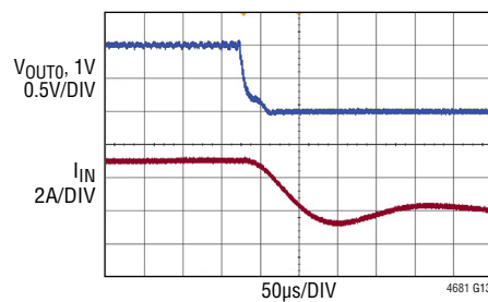
FIGURE 48 CIRCUIT, 12\text{V}_{\text{IN}} , 30\text{A} LOAD ON \text{V}_{\text{OUT0}} PRIOR TO APPLICATION OF SHORT-CIRCUIT USE HIGH RANGE OF \text{I} LIMIT SYSTEM SHORT-CIRCUIT USING LOW IMPEDANCE COPPER ACROSS OUTPUT (HARD SHORT)
