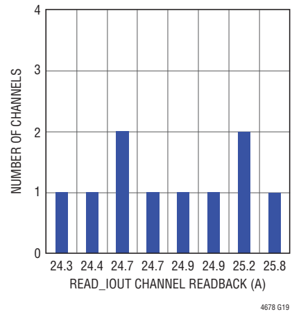
READ_IOUT of 10 LTM4678 Channels 12\text{V}_{\text{IN}} , 1\text{V}_{\text{OUT}} , T_J = 125^{\circ}\text{C} , I_{\text{OUT}n} = 25\text{A} , System Having Reached Thermally Steady-State Condition, No Airflow
