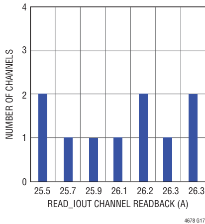
READ_IOUT of 10 LTM4678 Channels 12\text{V}_{\text{IN}} , 1\text{V}_{\text{OUT}} , T_J = -40^{\circ}\text{C} , I_{\text{OUT}n} = 25\text{A} , System Having Reached Thermally Steady-State Condition, No Airflow
