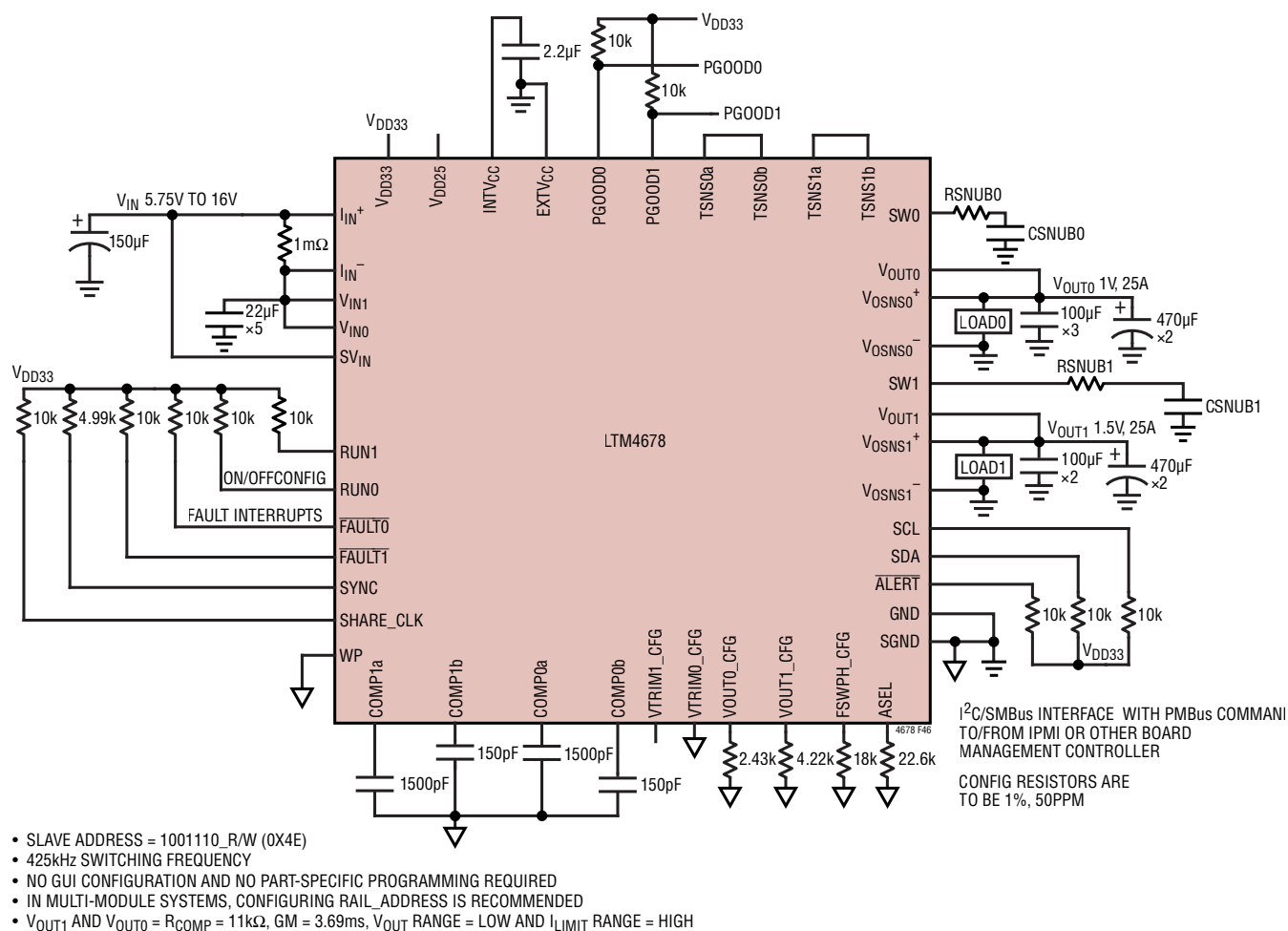
Figure 46. 1.0V and 1.5V Outputs at 25A With Providing I²C/SMBus/PMBus Serial Interface
