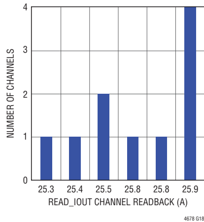
READ_IOUT of 10 LTM4678 Channels 12\text{V}_{\text{IN}} , 1\text{V}_{\text{OUT}} , T_J = 25^{\circ}\text{C} , I_{\text{OUT}n} = 25\text{A} , System Having Reached Thermally Steady-State Condition, No Airflow
