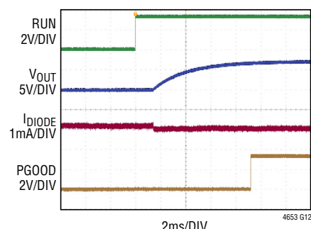
Start-Up, Pre-Bias
