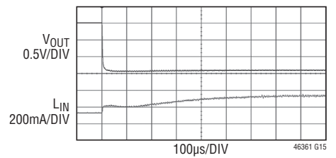
No-Load Short-Circuit
