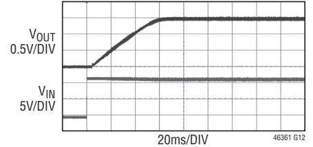
Start-Up with Soft-Start Full Load
