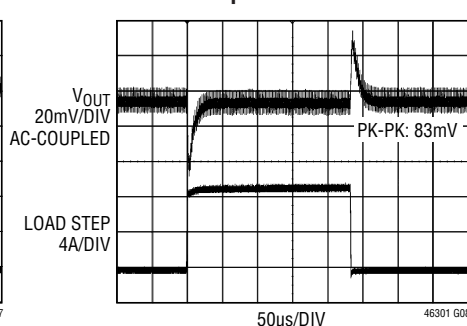
Dual Phase Single Output 25% (9A) Transient Response at 1.5V Output
