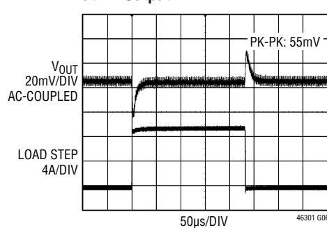
Dual Phase Single Output 25% (9A) Transient Response at 1V Output
