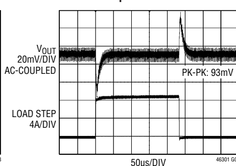
Dual Phase Single Output 25% (9A) Transient Response at 1.8V Output
