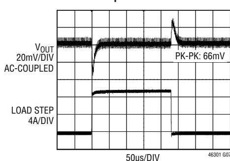
Dual Phase Single Output 25% (9A) Transient Response at 1.2V Output
