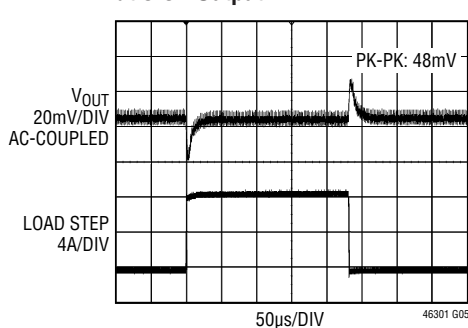
Dual Phase Single Output 25% (9A) Transient Response at 0.9V Output
