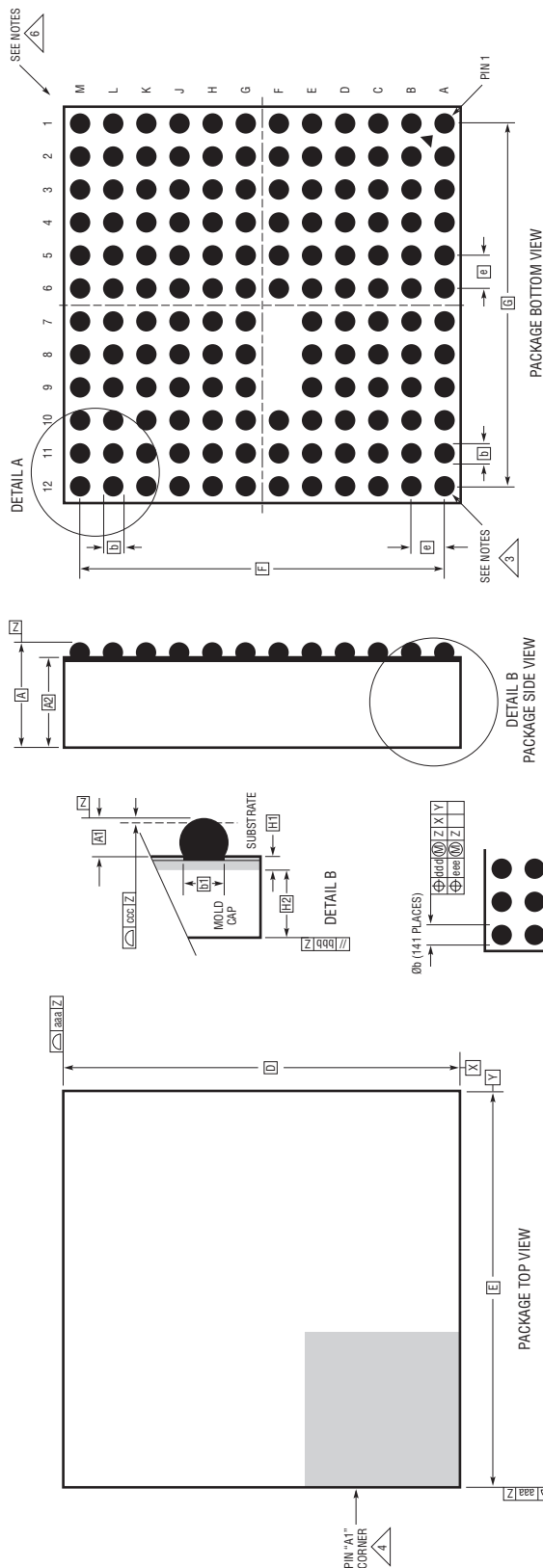
BGA Package 141-Lead (15mm × 15mm × 3.42mm) (Reference LTC DWG # 05-08-1899 Rev D)
