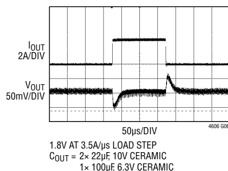
1.8V Transient Response
