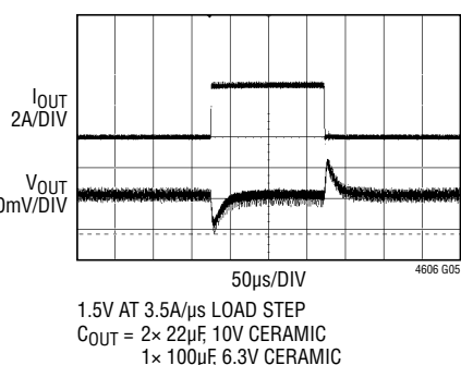
1.5V Transient Response
