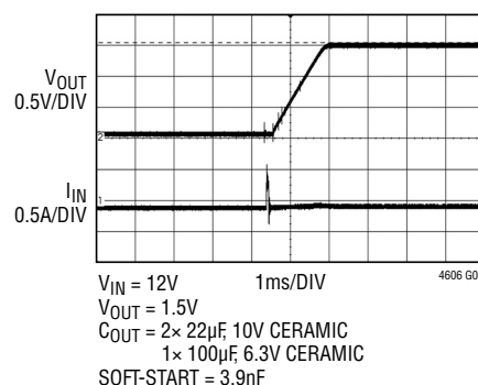
-55°C, Start-Up, I OUT = 0A
