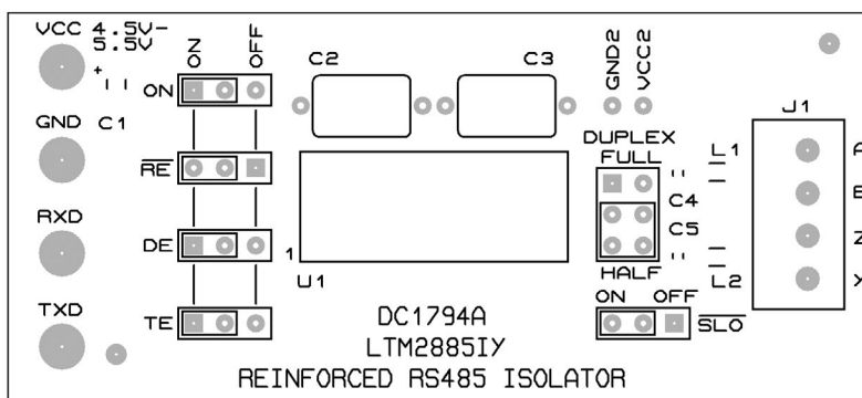
Figure 16a. LTM2885 Demo Board Layout
