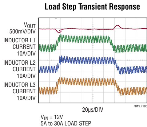
Figure 10. High Efficiency 380kHz 3-Phase 5V/50A Regulator
