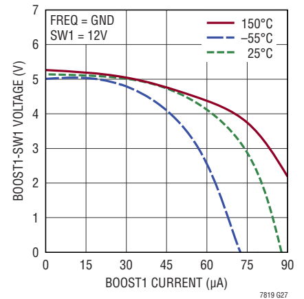
BOOST1-SW1 Charge Pump Voltage vs BOOST1 Current
