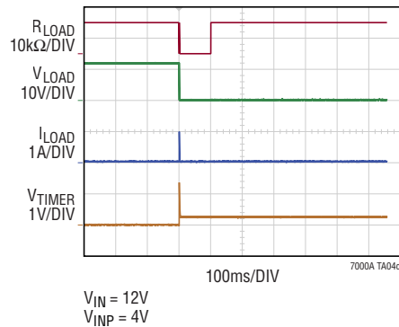
R_{\text{TIMER}} = 100k 12Ω/100ms LOAD PULSE
