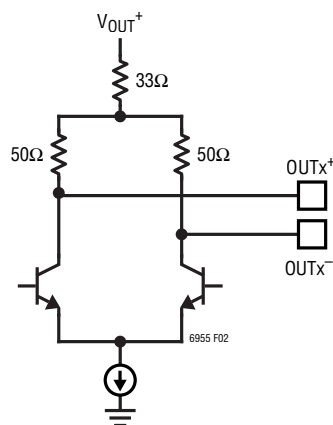
Figure 2. Simplified CML Interface Schematic (All OUTx)
