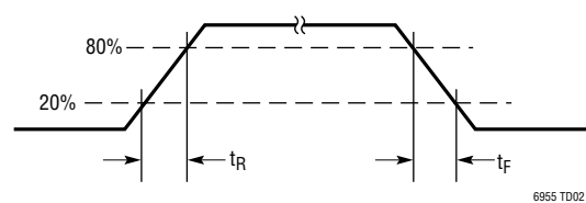
Differential CML Rise/Fall Times
