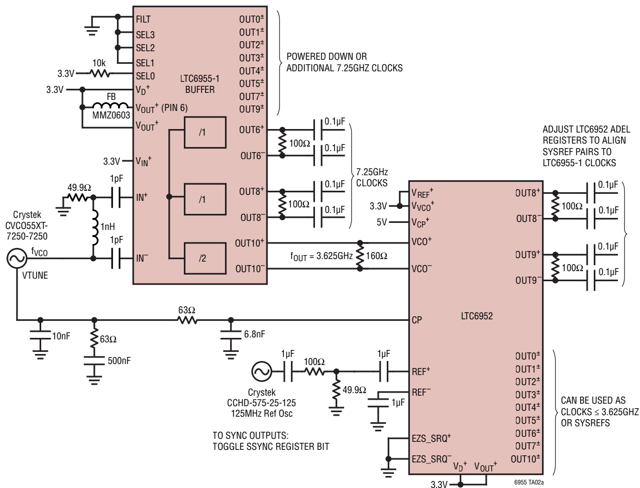
7.25GHz JESD204B CLK to SYSREF Alignment Calibration Over Temperature
