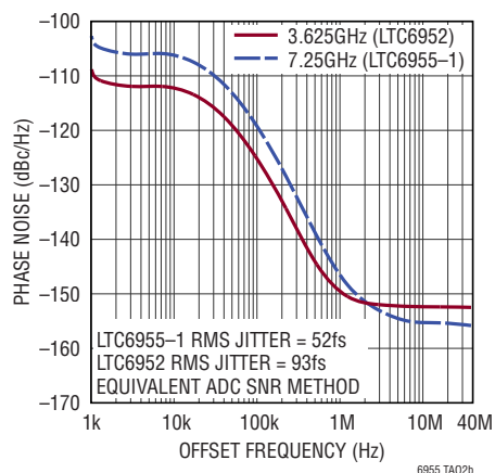
LTC6955-1 and LTC6952 Phase Noise f_{\text{VCO}} = 7.25\text{GHz}
