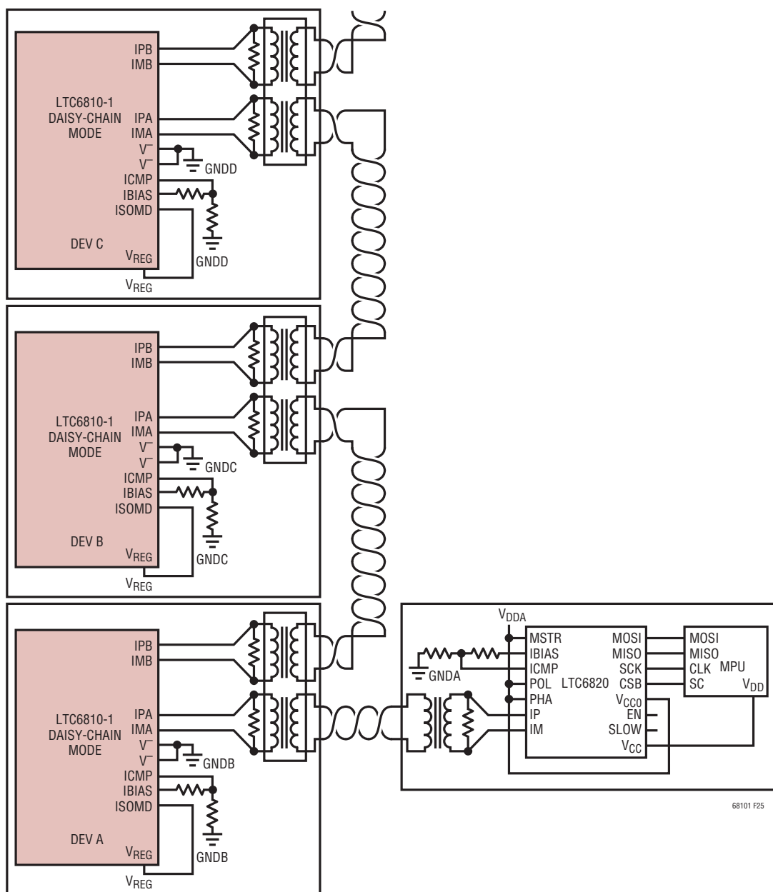
Figure 25. Transformer-Coupled Daisy-Chain Configuration Using LT6810-1
